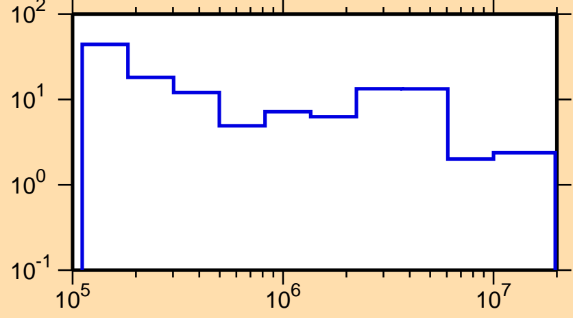
\Delta\sigma/\sigma vs. E for ^{177}\text{Lu}(n,\text{tot.})
