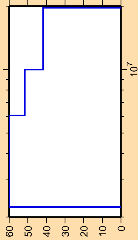
\Delta\sigma/\sigma vs. E for ^{177}\text{Lu}(n,p)
