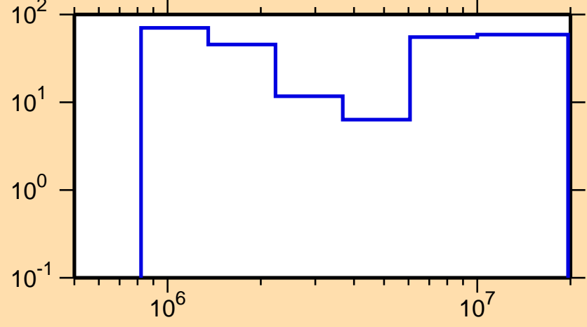
\Delta\sigma/\sigma vs. E for ^{177}\text{Lu}(n,ncont.)
