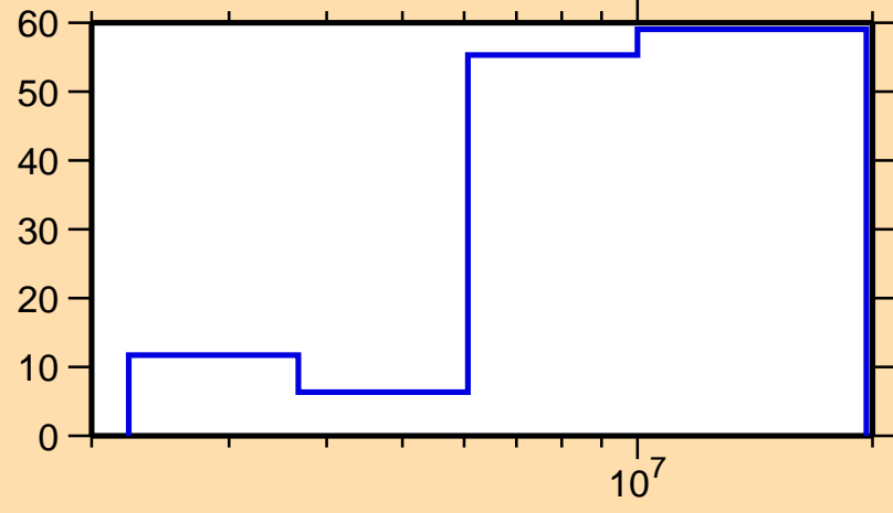
\Delta\sigma/\sigma vs. E for ^{177}\text{Lu}(n,ncont.)
