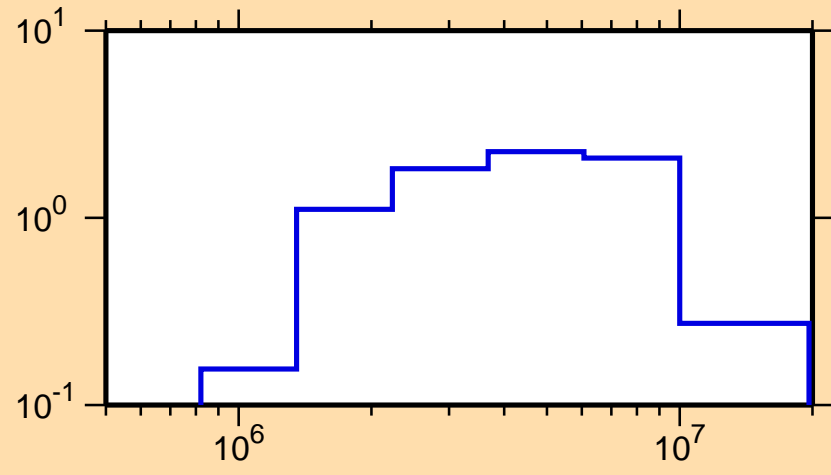
\sigma vs. E for ^{177}\text{Lu}(n,n\text{cont.})
