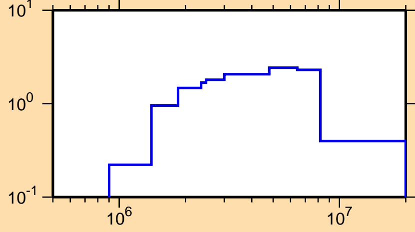
\sigma vs. E for ^{177}\text{Lu}(n,n\text{cont.})
