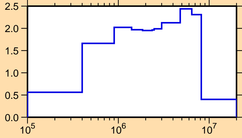
\sigma vs. E for ^{177}\text{Lu}(n,\text{inel.})
