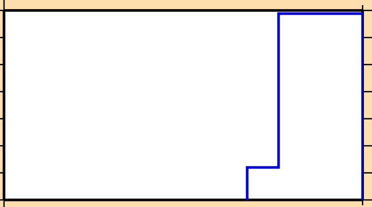
\sigma vs. E for ^{177}\text{Lu}(n,p\alpha)
