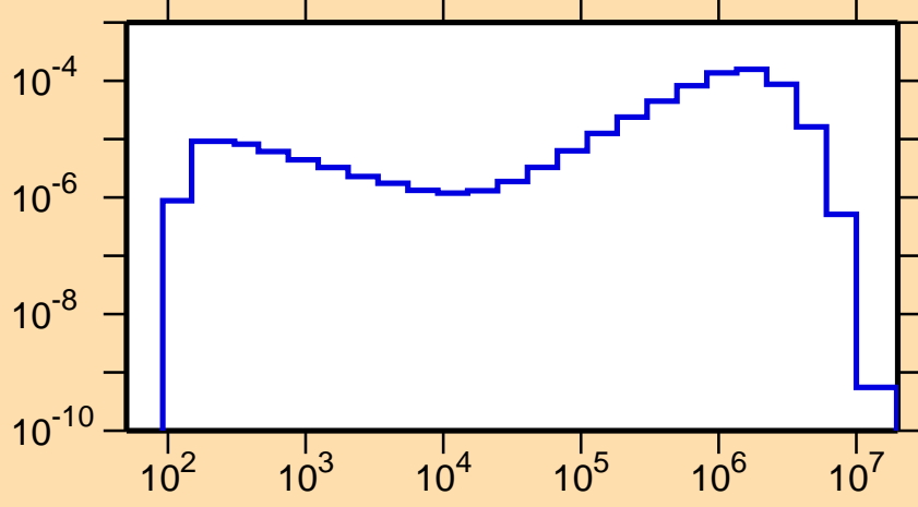
\sigma vs. E for ^{177}\text{Lu}(n,n_2)
