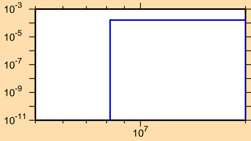
\sigma vs. E for ^{177}\text{Lu}(n,t)
