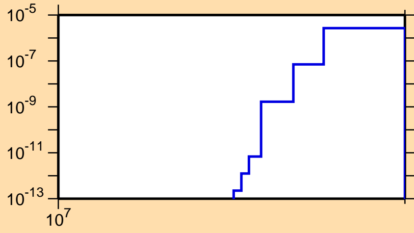
\sigma vs. E for ^{178}\text{Lu}(n,2np)
