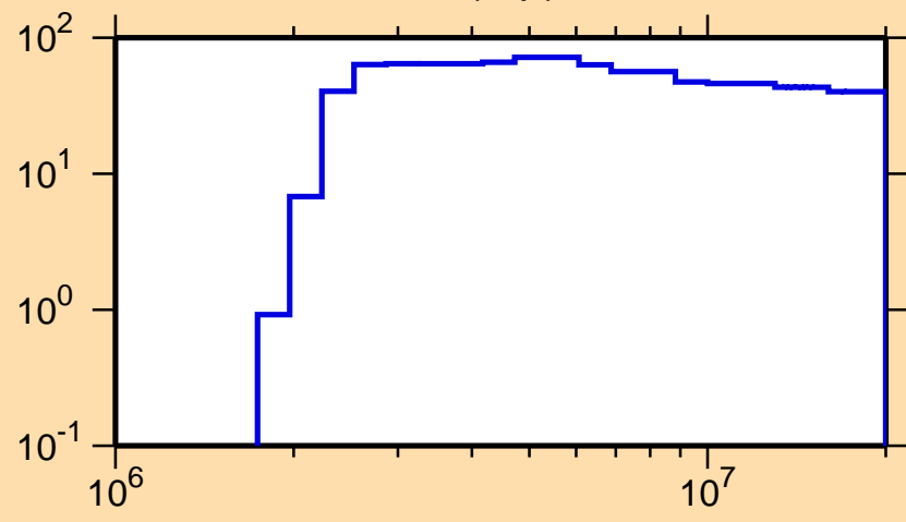
\Delta\sigma/\sigma vs. E for ^{178}\text{Lu}(n,p)
