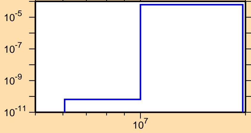
\sigma vs. E for ^{178}\text{Lu}(n,t)
