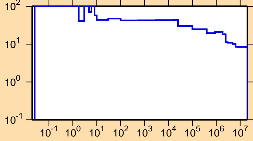
\Delta\sigma/\sigma vs. E for ^{178}\text{Lu}(n,\text{nonel.})
