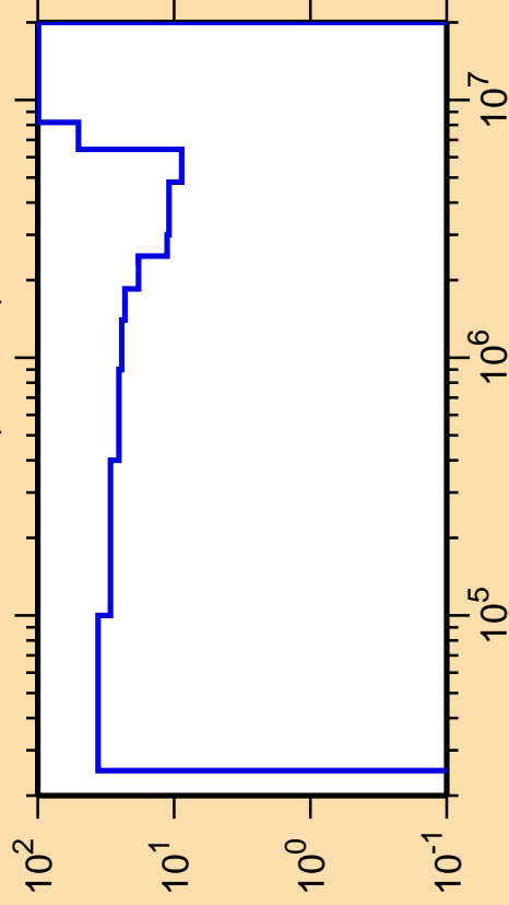
\Delta\sigma/\sigma vs. E for ^{178}\text{Lu}(n,\text{inel.})
