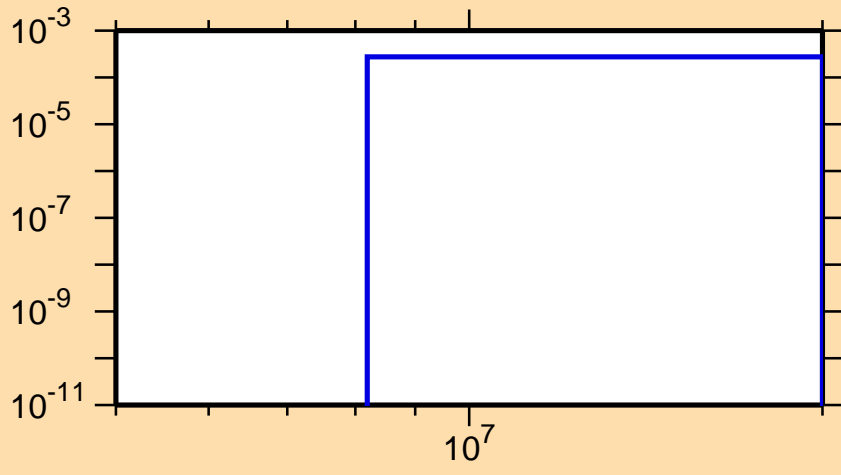
\sigma vs. E for ^{178}\text{Lu}(n,d)
