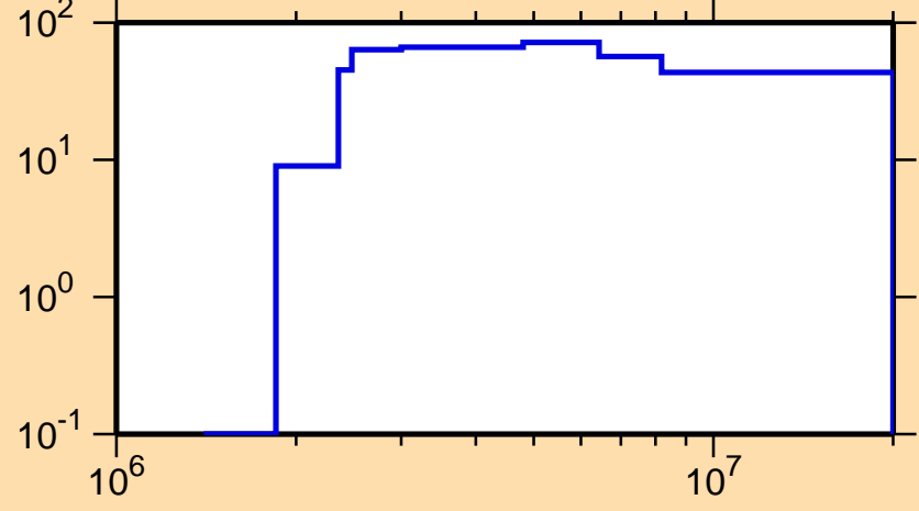
\Delta\sigma/\sigma vs. E for ^{178}\text{Lu}(n,p)
