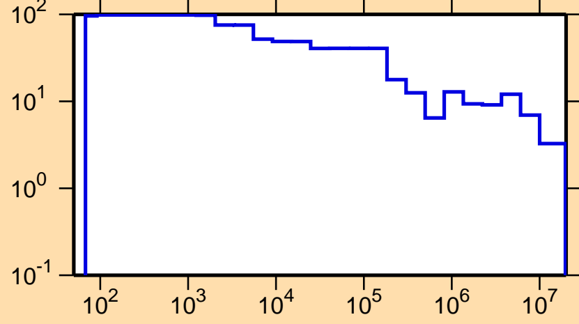
\Delta\sigma/\sigma vs. E for ^{178}\text{Lu}(n,\text{tot.})
