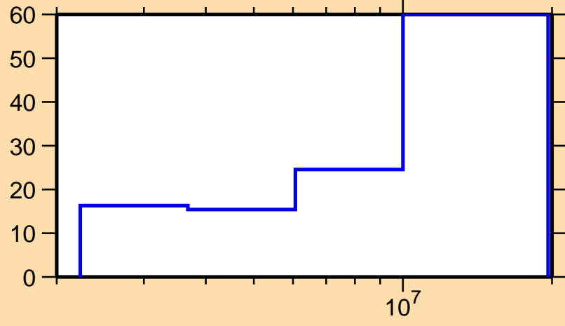
\Delta\sigma/\sigma vs. E for ^{178}\text{Lu}(n,ncont.)
