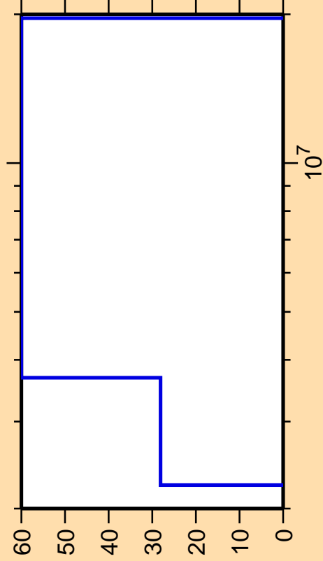
\Delta\sigma/\sigma vs. E for ^{178}\text{Lu}(n,p)
