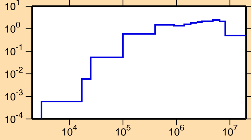
\sigma vs. E for ^{178}\text{Lu}(n,\text{inel.})
