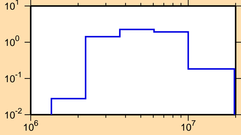
\sigma vs. E for ^{179}\text{Lu}(n,n\text{cont.})
