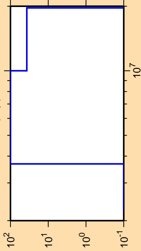
\Delta\sigma/\sigma vs. E for ^{179}\text{Lu}(n,p)
