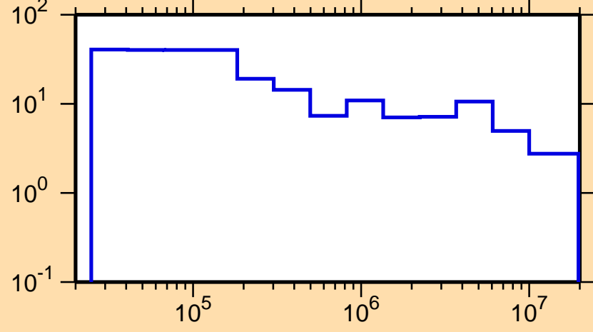
\Delta\sigma/\sigma vs. E for ^{179}\text{Lu}(n,\text{tot.})
