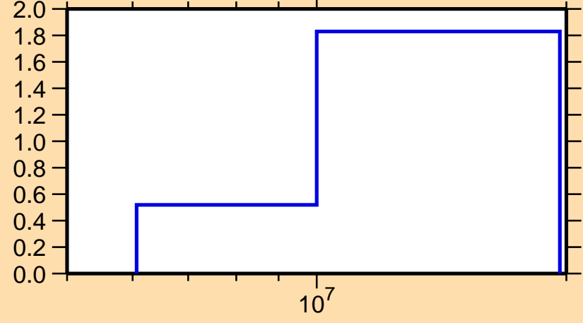
\sigma vs. E for ^{179}\text{Lu}(n,2n)
