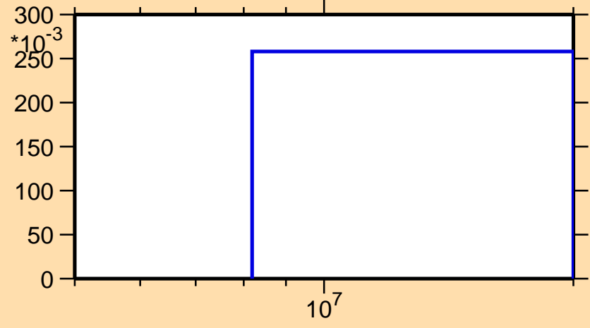
\sigma vs. E for ^{179}\text{Lu}(n,3n)
