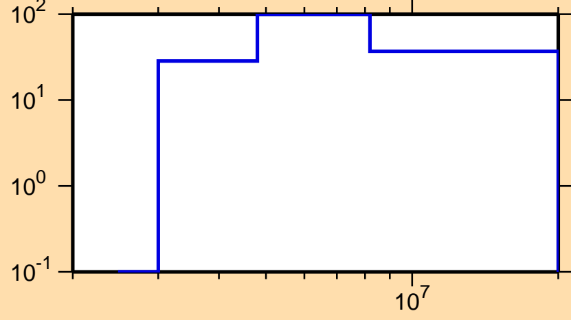
\Delta\sigma/\sigma vs. E for ^{179}\text{Lu}(n,p)
