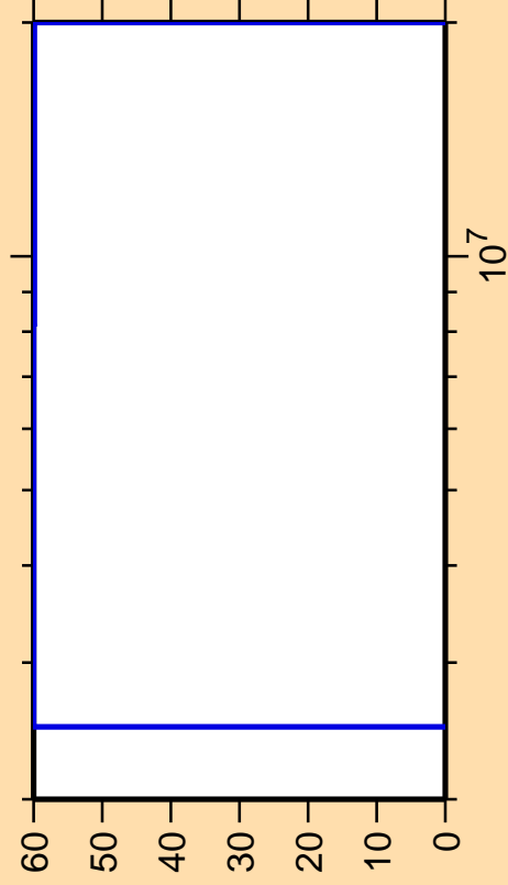
\Delta\sigma/\sigma vs. E for ^{179}\text{Lu}(n,\alpha)
