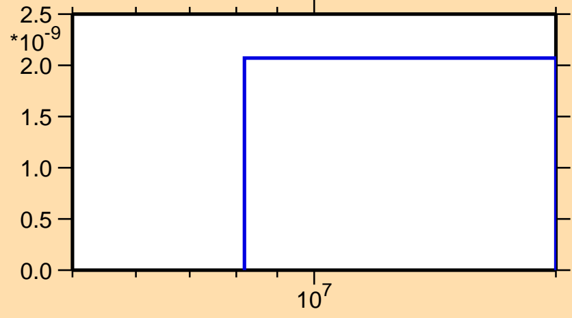
\sigma vs. E for ^{179}\text{Lu}(n,2n\alpha)
