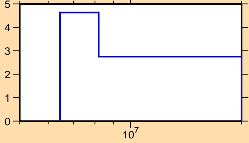
\Delta\sigma/\sigma vs. E for ^{179}\text{Lu}(n,\text{tot.})
