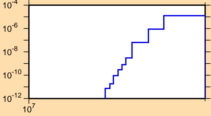
\sigma vs. E for ^{180}\text{Lu}(n,nd)
