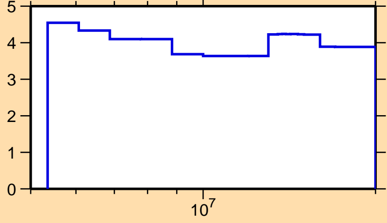
\Delta\sigma/\sigma vs. E for ^{180}\text{Lu}(n,\text{nonel.})
