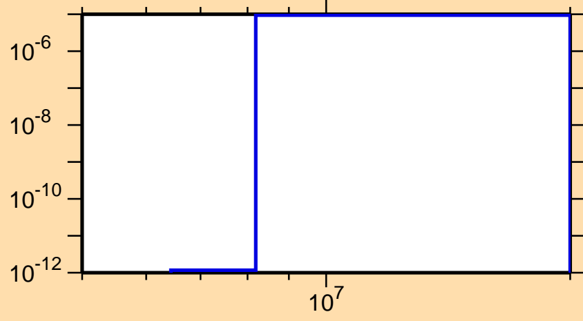
\sigma vs. E for ^{181}\text{Lu}(n,n\alpha)
