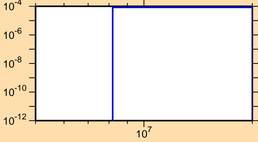
\sigma vs. E for ^{181}\text{Lu}(n,d)
