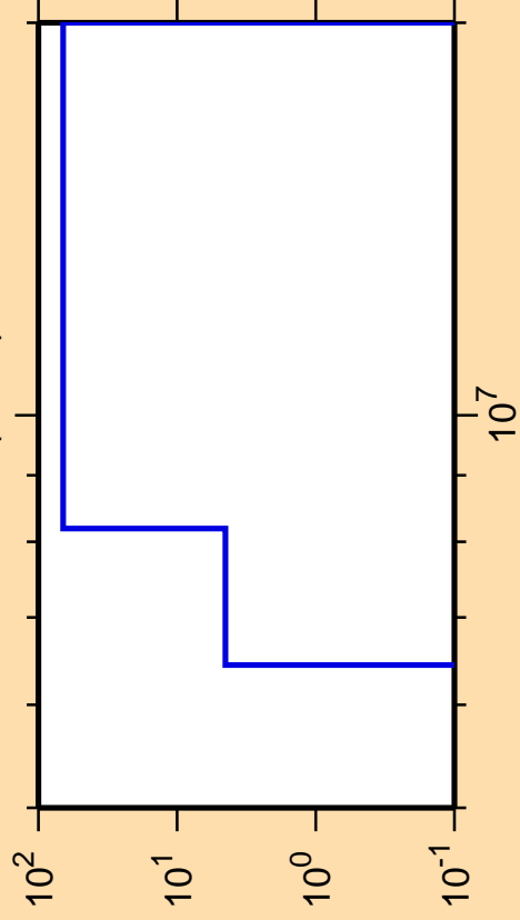
\Delta\sigma/\sigma vs. E for ^{181}\text{Lu}(n,n\alpha)
