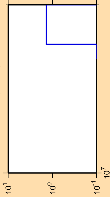
\Delta\sigma/\sigma vs. E for ^{182}\text{Lu}(n,3n\alpha)
