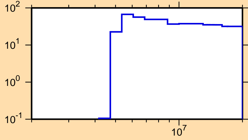
\Delta\sigma/\sigma vs. E for ^{182}\text{Lu}(n,p)
