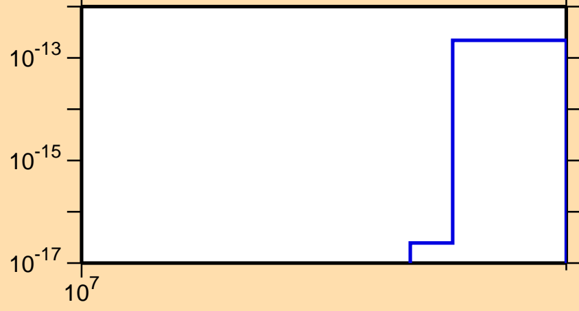
\sigma vs. E for ^{182}\text{Lu}(n,3n\alpha)
