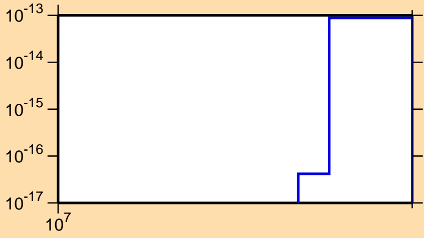
\sigma vs. E for ^{182}\text{Lu} (mt 11)
