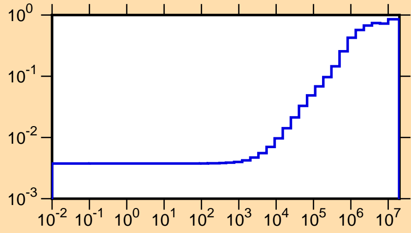
\mu vs. E for ^{182}\text{Lu}(\text{mt251})
