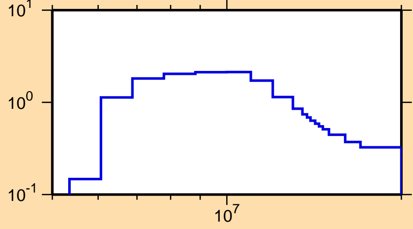
\sigma vs. E for ^{185}\text{Lu}(n,2n)
