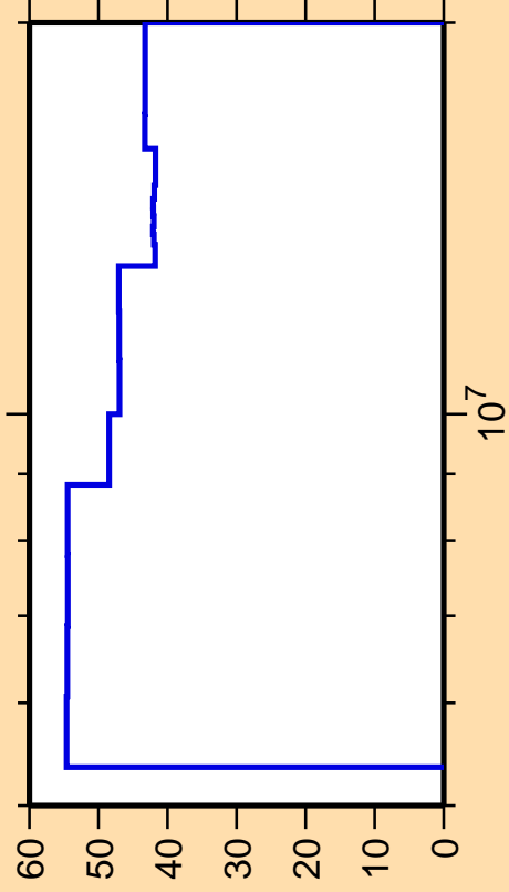
\Delta\sigma/\sigma vs. E for ^{185}\text{Lu}(n,n_1)
