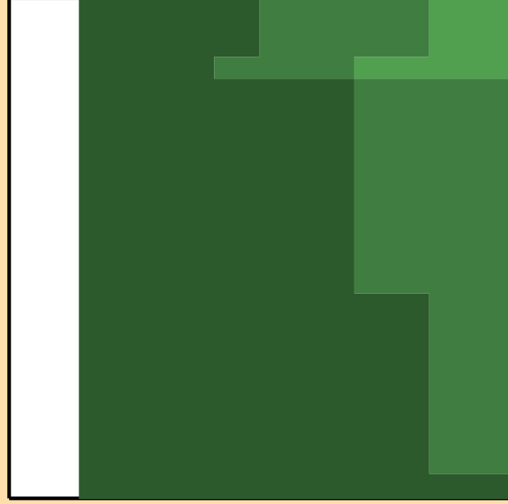
\Delta\sigma/\sigma vs. E for ^{185}\text{Lu}(n,p)
