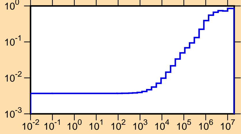
\mu vs. E for ^{185}\text{Lu}(\text{mt251})
