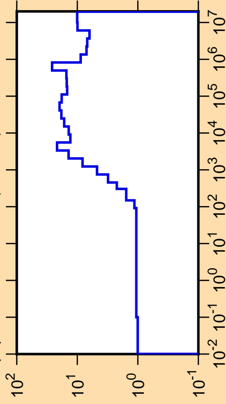
\Delta\mu/\mu vs. E for ^{185}\text{Lu}(\text{mt251})
