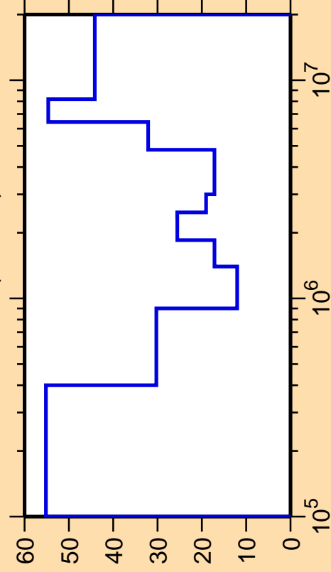
\Delta\sigma/\sigma vs. E for ^{185}\text{Lu}(n,\text{inel.})
