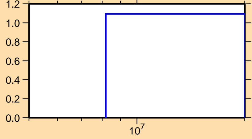
\sigma vs. E for ^{185}\text{Lu}(n,3n)
