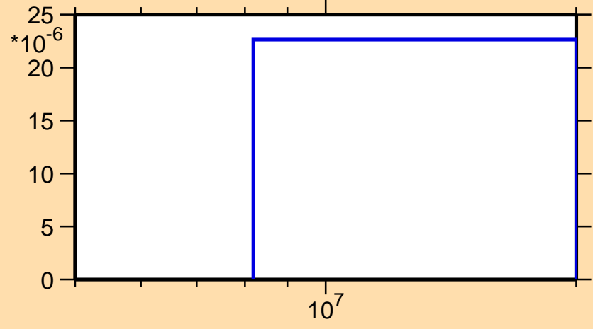
\sigma vs. E for ^{185}\text{Lu}(n,d)
