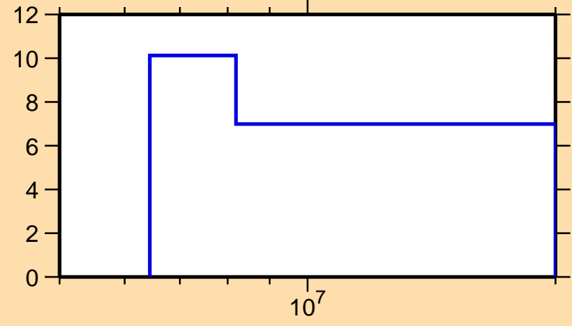
\Delta\sigma/\sigma vs. E for ^{185}\text{Lu}(n,el.)
