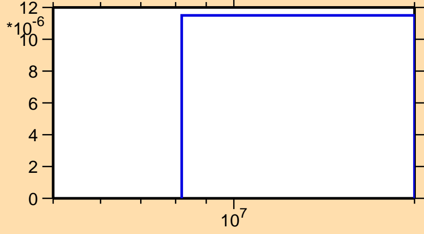
\sigma vs. E for ^{185}\text{Lu}(n,t)
