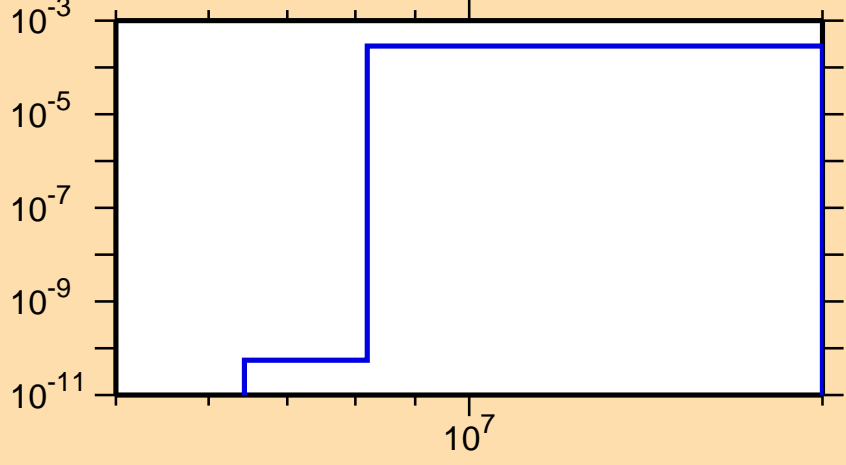
\sigma vs. E for ^{185}\text{Lu}(n,p)
