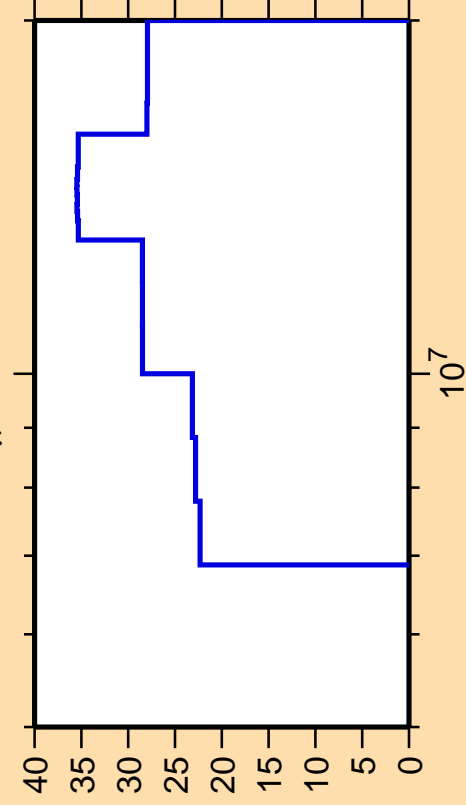
\Delta\sigma/\sigma vs. E for ^{291}\gamma
