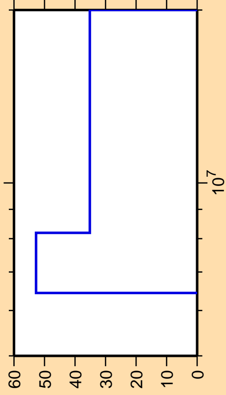
\Delta\sigma/\sigma vs. E for ^{291}\alpha
