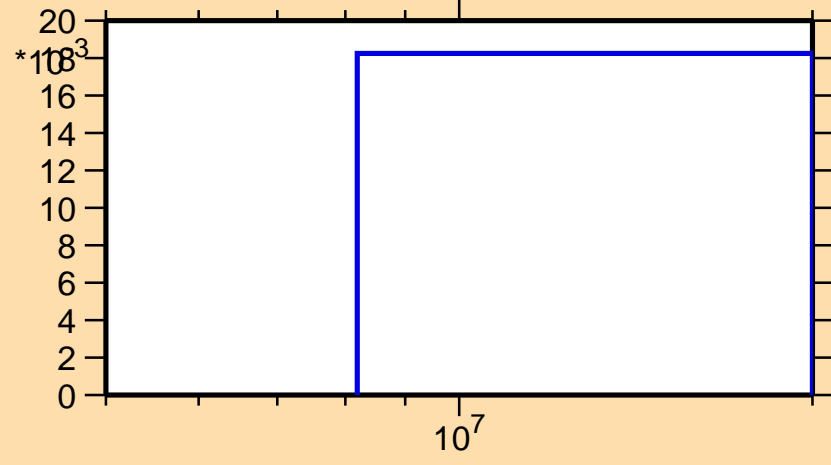
\sigma vs. E for ^{291}\alpha
