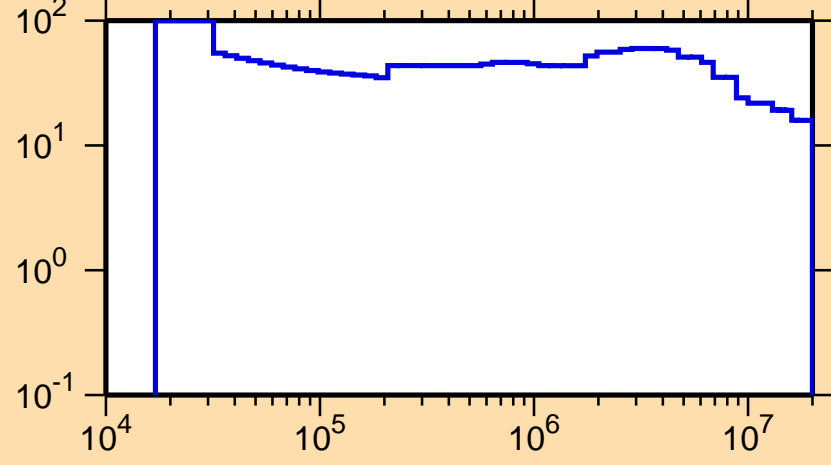
\Delta\sigma/\sigma vs. E for ^{246}\text{Md}(n,f)
