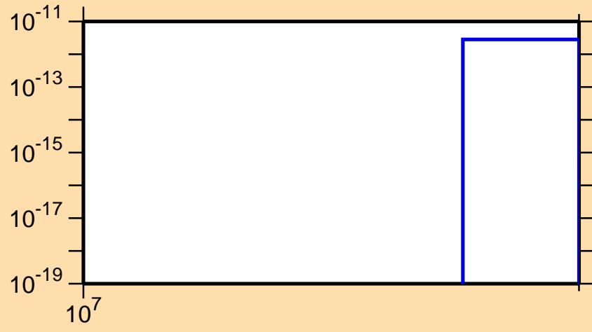
\sigma vs. E for ^{246}\text{Md} (mt 42)
