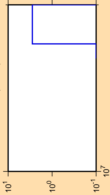
\Delta\sigma/\sigma vs. E for ^{246}\text{Md} (mt 42)
