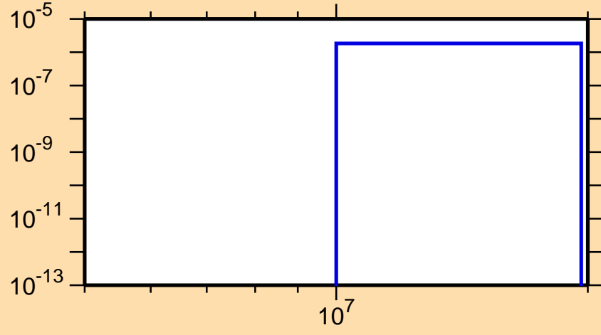
\sigma vs. E for ^{246}\text{Md}(n,2np)
