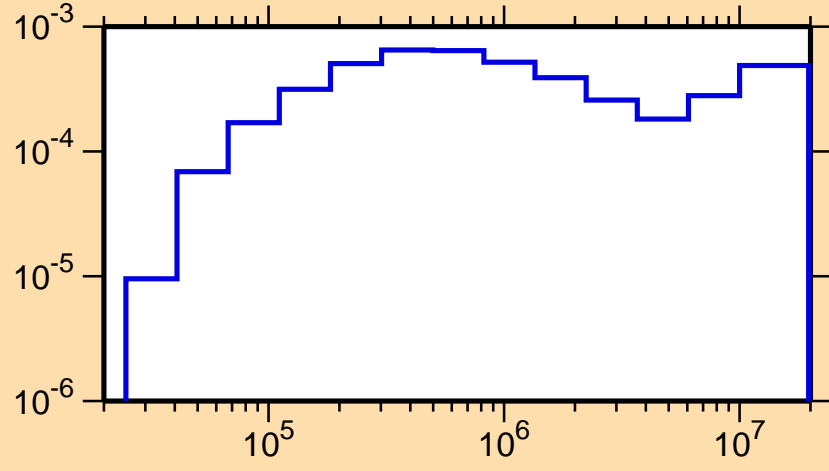
\sigma vs. E for ^{246}\text{Md}(n,\alpha)
