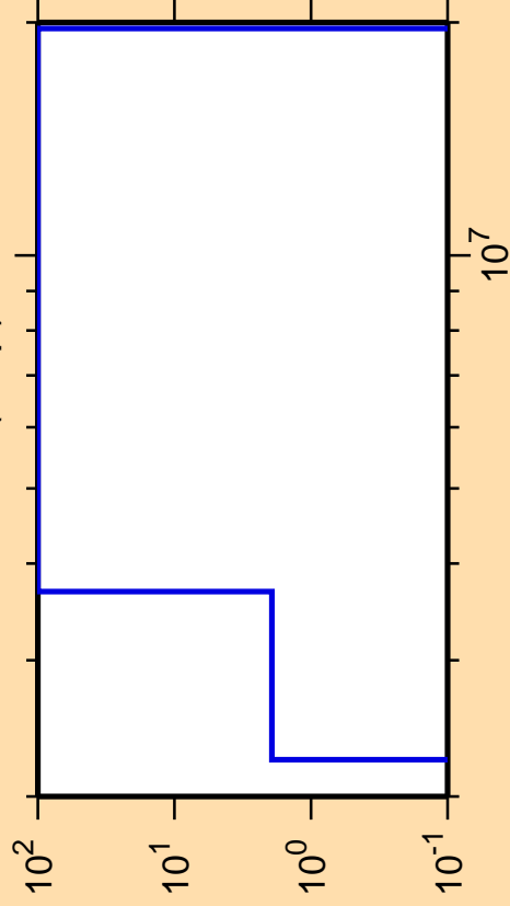
\Delta\sigma/\sigma vs. E for ^{246}\text{Md}(n,np)
