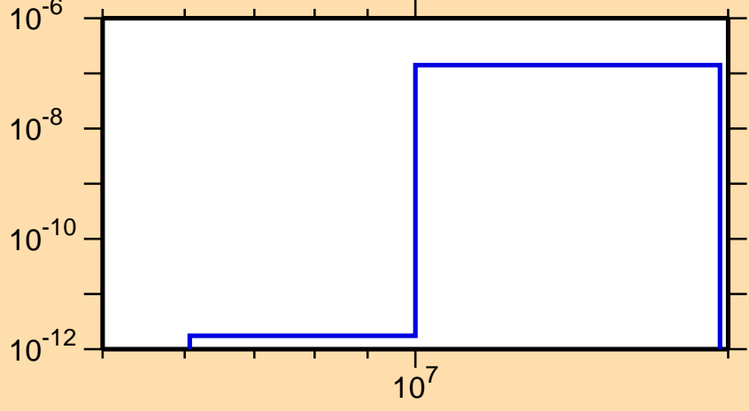
\sigma vs. E for ^{246}\text{Md}(n,\text{He3})
