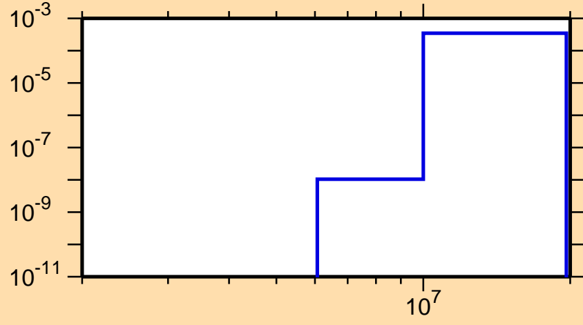
\sigma vs. E for ^{246}\text{Md}(n,t)
