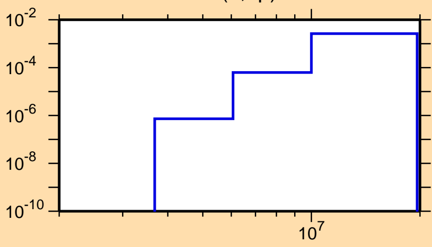
\sigma vs. E for ^{246}\text{Md}(n,np)
