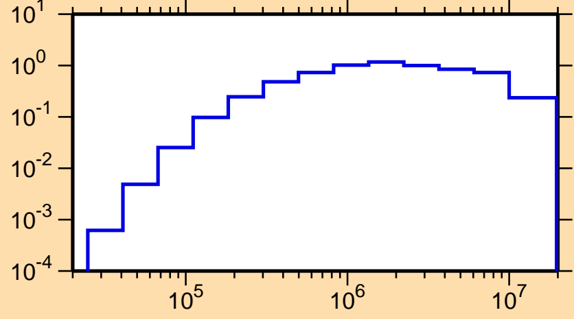
\sigma vs. E for ^{246}\text{Md}(n,n\text{cont.})
