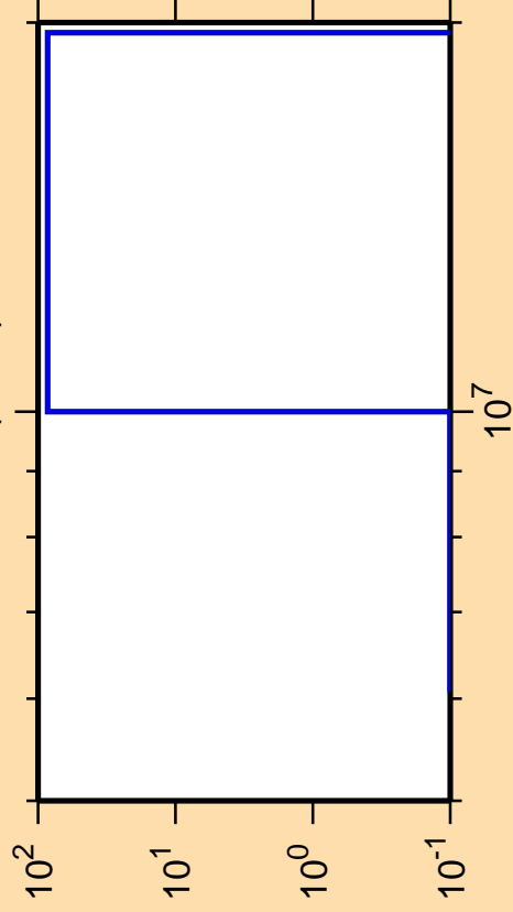
\Delta\sigma/\sigma vs. E for ^{246}\text{Md}(n,\text{nd})
