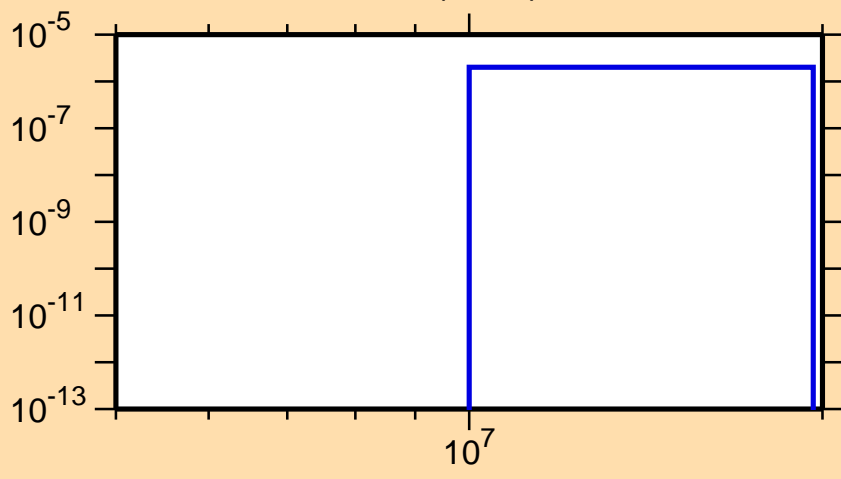
\sigma vs. E for ^{246}\text{Md}(n,\text{nd})
