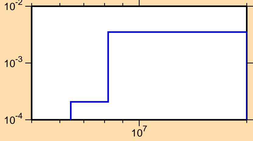
\sigma vs. E for ^{246}\text{Md}(n,2n\alpha)
