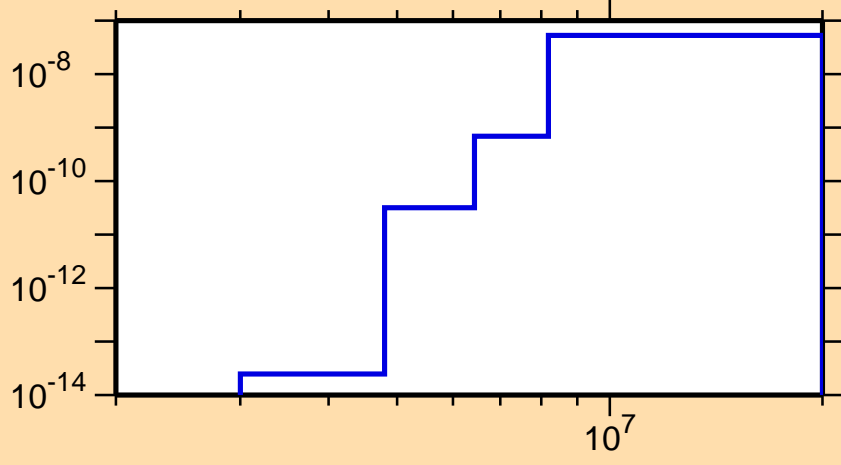
\sigma vs. E for ^{246}\text{Md} (mt 45)
