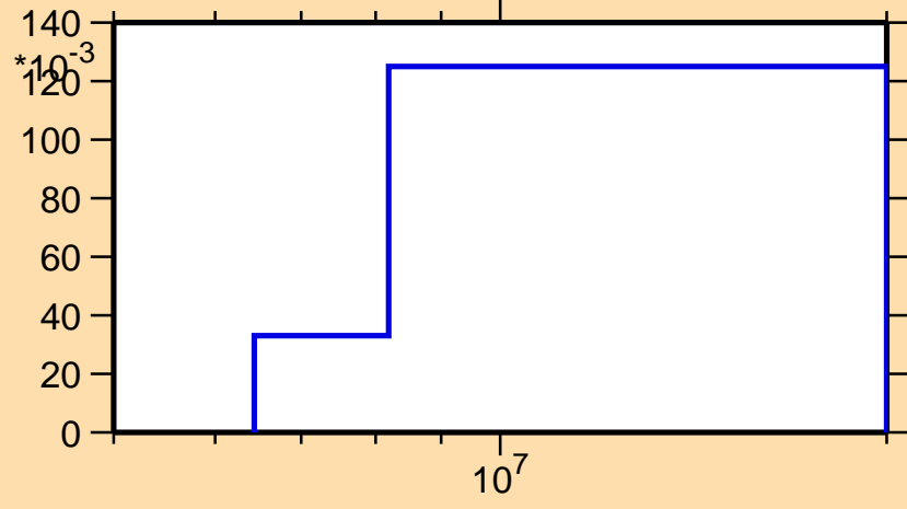
\sigma vs. E for ^{246}\text{Md}(n,2n)
