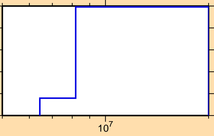
\sigma vs. E for ^{246}\text{Md}(\text{mt117})
