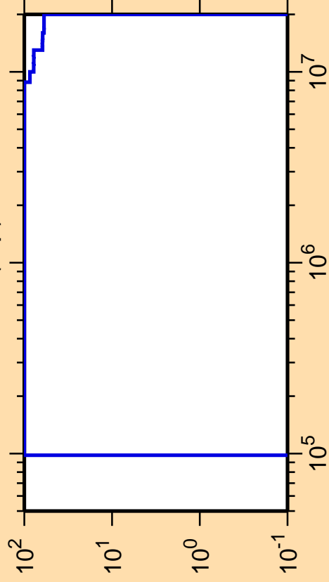
\Delta\sigma/\sigma vs. E for ^{247}\text{Md}(n,p)
