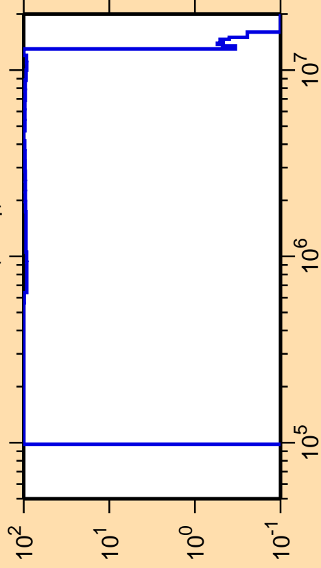
\Delta\sigma/\sigma vs. E for ^{247}\text{Md}(n,n_1)
