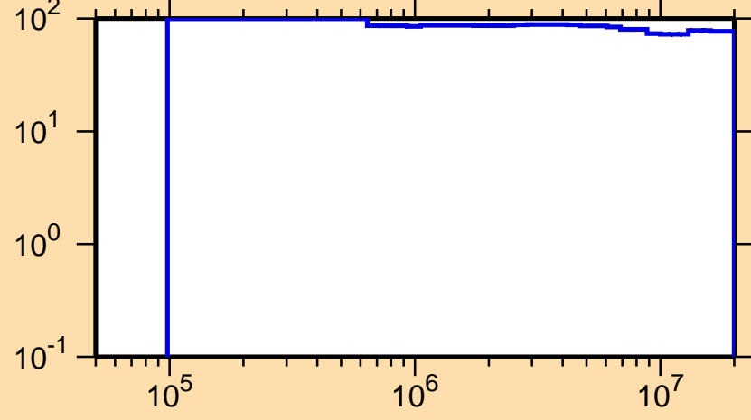
\Delta\sigma/\sigma vs. E for ^{247}\text{Md}(n,ncont.)
