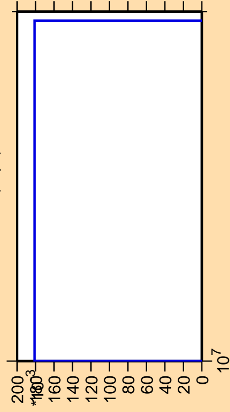
\Delta\sigma/\sigma vs. E for ^{247}\text{Md}(n,\text{pt})
