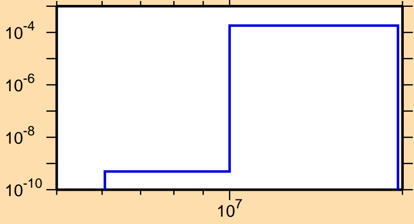
\sigma vs. E for ^{247}\text{Md}(n,t)
