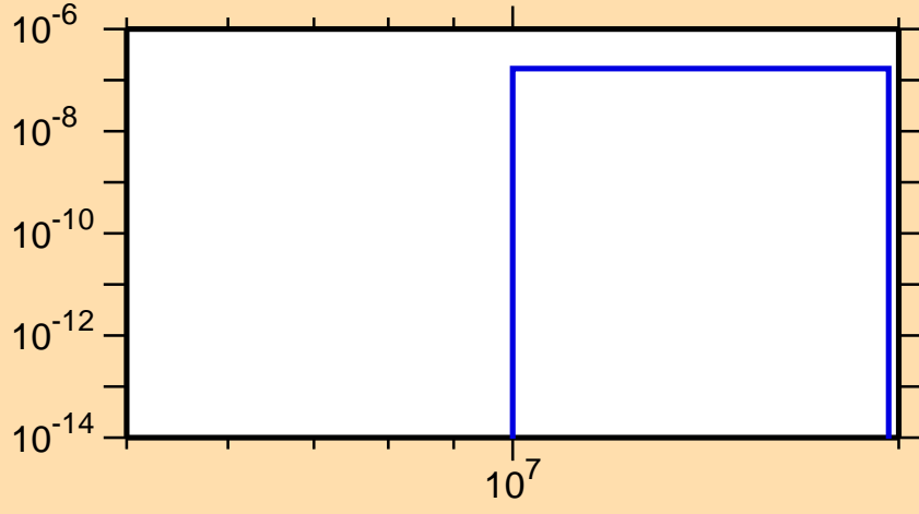
\sigma vs. E for ^{247}\text{Md}(n,\text{nd})
