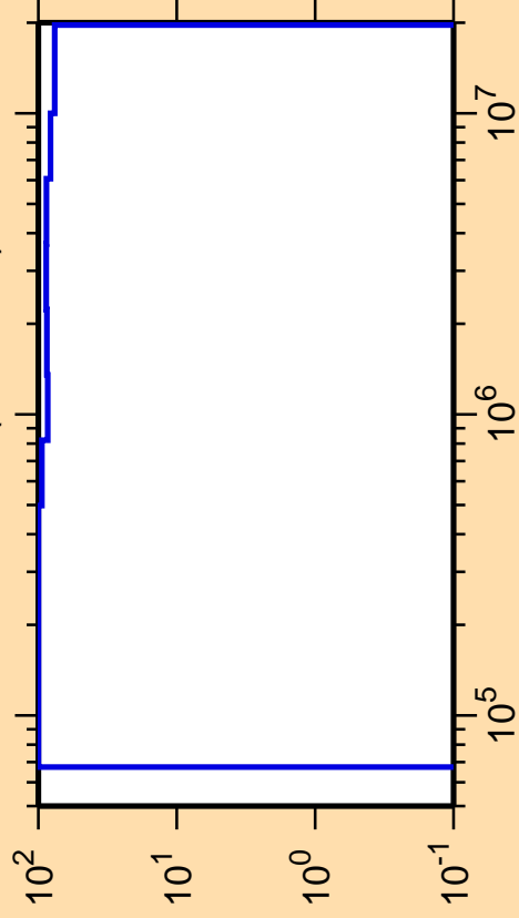
\Delta\sigma/\sigma vs. E for ^{247}\text{Md}(n, n_{\text{cont}})
