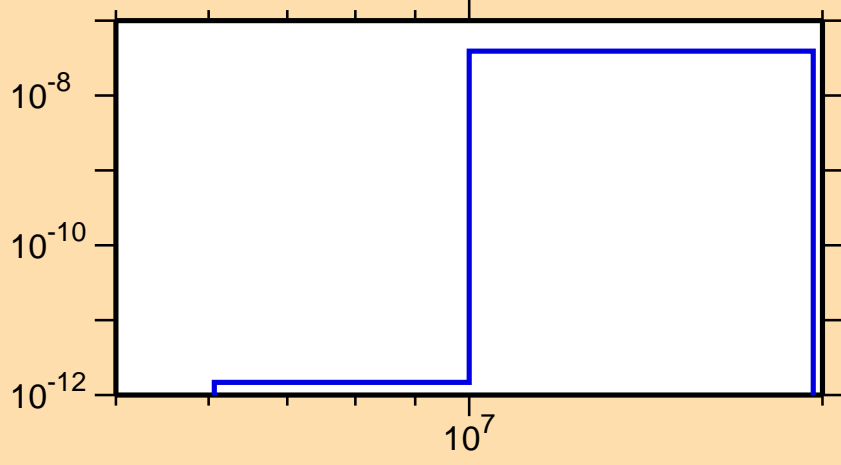
\sigma vs. E for ^{247}\text{Md} (mt 45)
