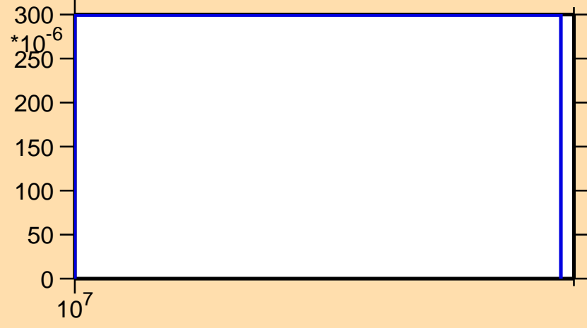
\sigma vs. E for ^{247}\text{Md}(n,3n)
