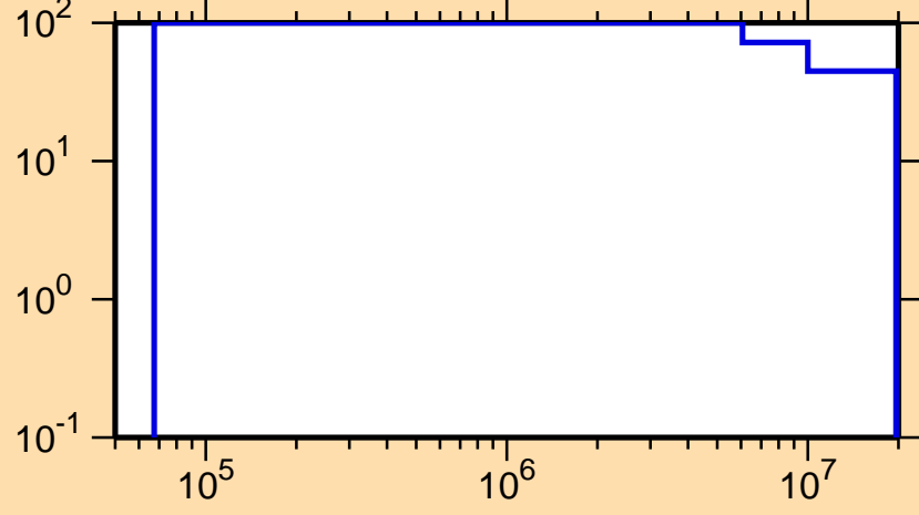
\Delta\sigma/\sigma vs. E for ^{247}\text{Md}(n,\text{f})
