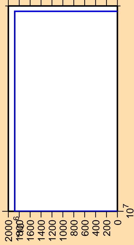
\Delta\sigma/\sigma vs. E for ^{247}\text{Md} (mt 11)
