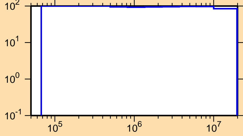
\Delta\sigma/\sigma vs. E for ^{247}\text{Md}(n, n_1)
