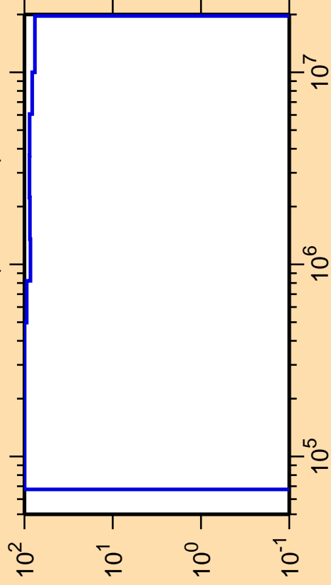
\Delta\sigma/\sigma vs. E for ^{247}\text{Md}(n,\text{ncont.})
