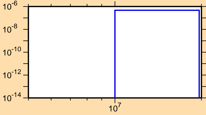
\sigma vs. E for ^{247}\text{Md}(n,2np)
