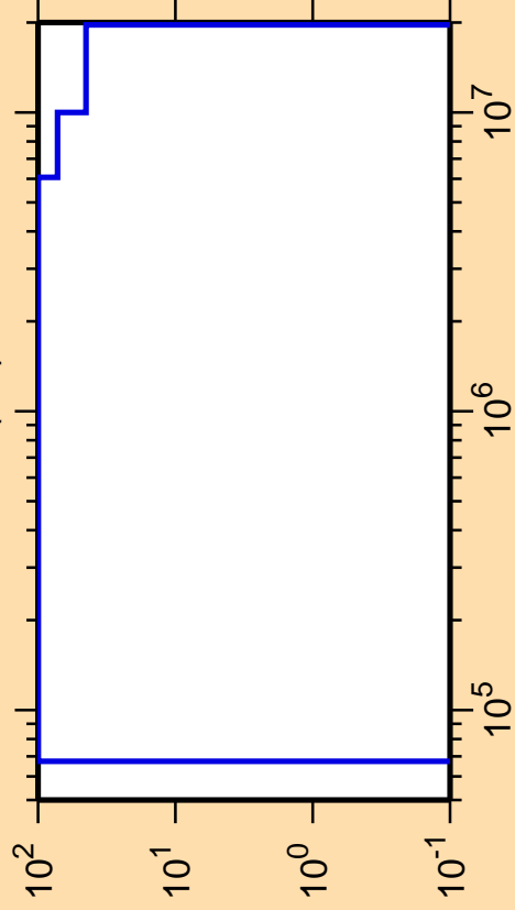
\Delta\sigma/\sigma vs. E for ^{247}\text{Md}(n,f)
