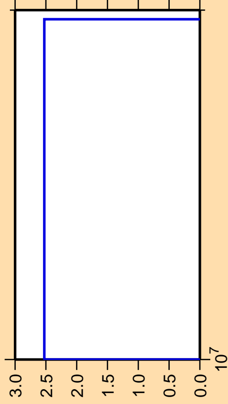
\Delta\sigma/\sigma vs. E for ^{247}\text{Md} (mt 34)
