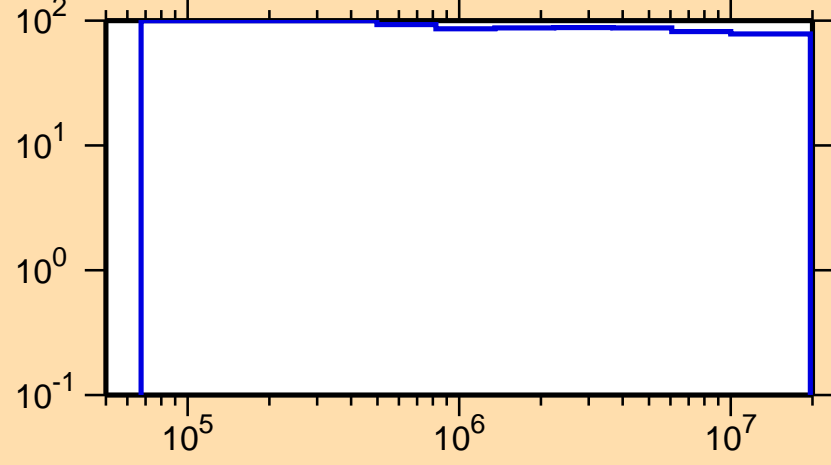
\Delta\sigma/\sigma vs. E for ^{247}\text{Md}(n,\text{inel.})
