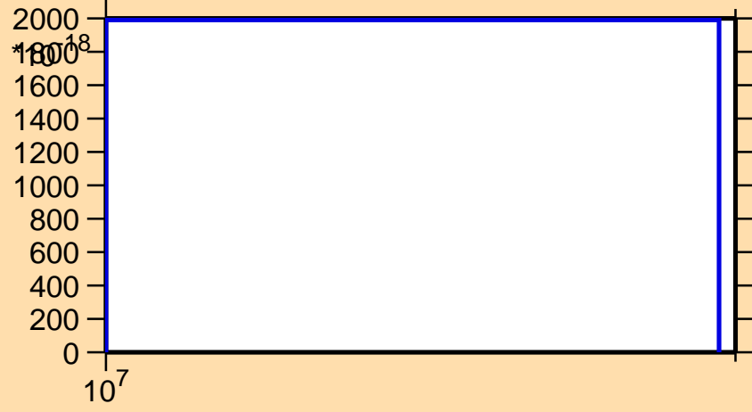
\sigma vs. E for ^{247}\text{Md} (mt 11)
