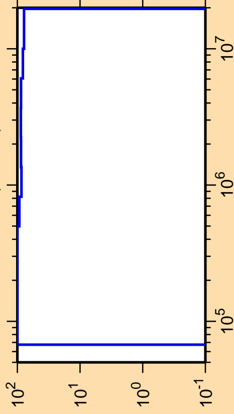
\Delta\sigma/\sigma vs. E for ^{247}\text{Md}(n,\text{inel.})
