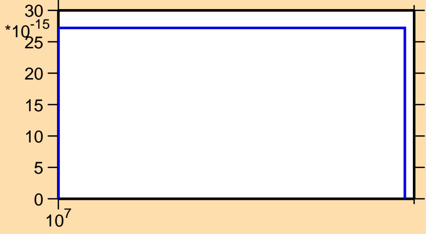
\sigma vs. E for ^{247}\text{Md}(n,\text{pt})
