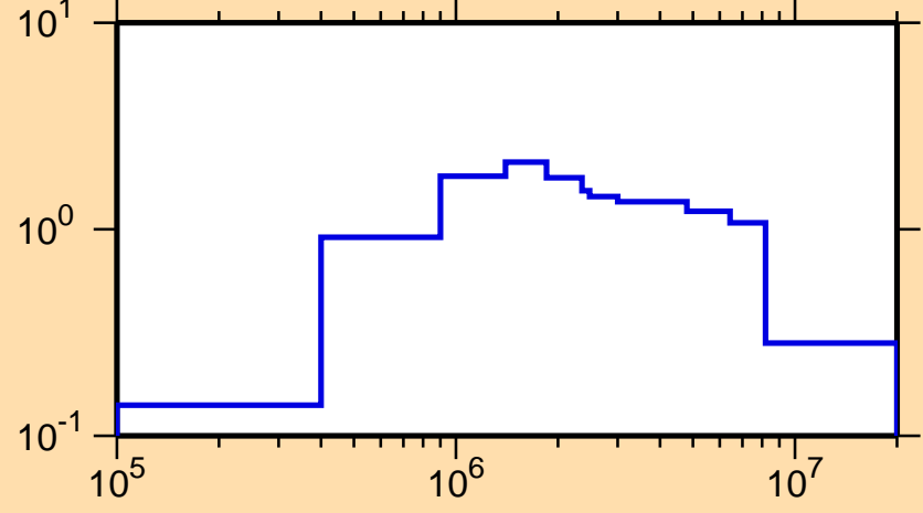
\sigma vs. E for ^{247}\text{Md}(n,\text{inel.})
