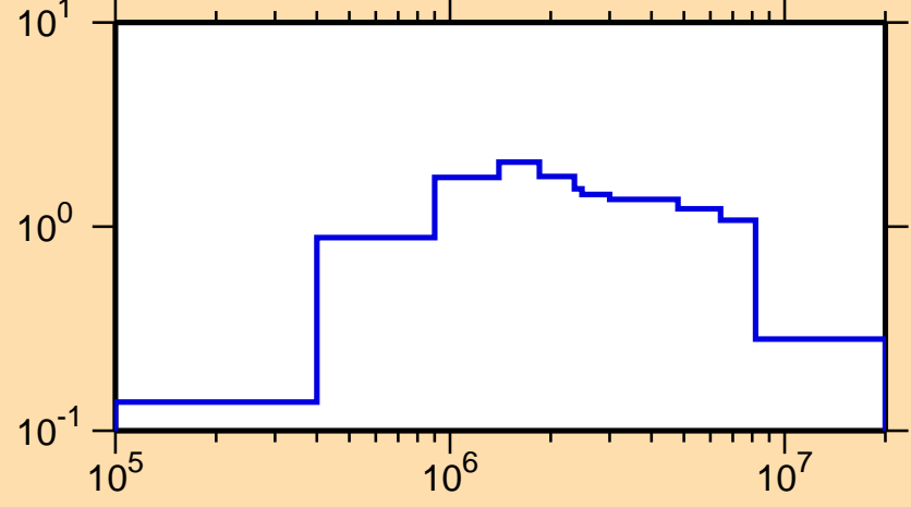
\sigma vs. E for ^{247}\text{Md}(n,n\text{cont.})
