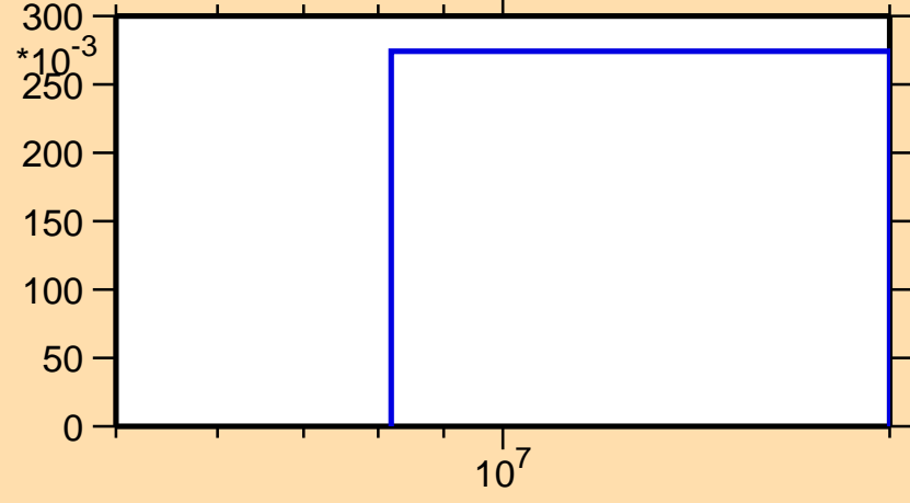
\sigma vs. E for ^{247}\text{Md}(n,2n)
