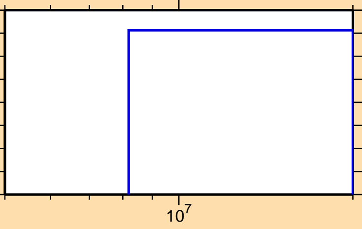
\sigma vs. E for ^{247}\text{Md}(n,\text{He3})
