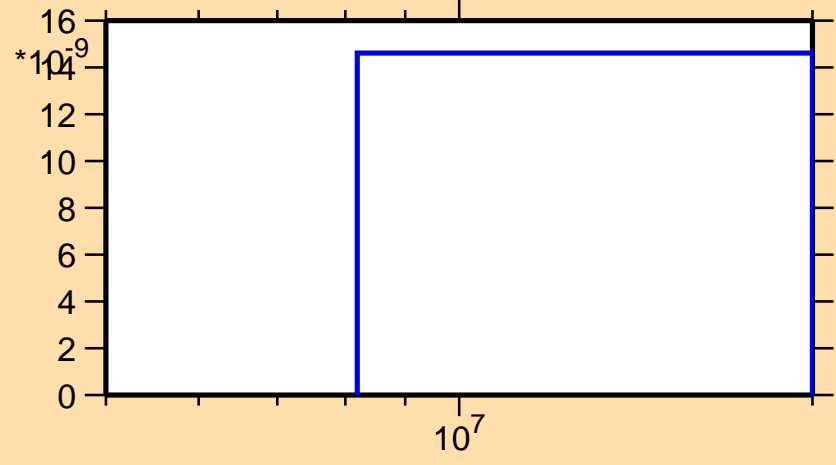
\sigma vs. E for ^{247}\text{Md}(n,nt)
