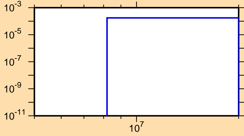
\sigma vs. E for ^{247}\text{Md}(n,2n\alpha)
