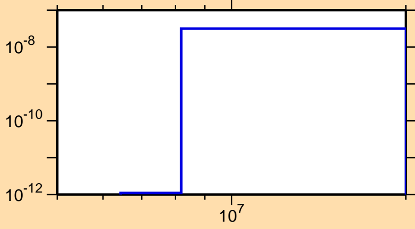
\sigma vs. E for ^{247}\text{Md}(\text{mt } 45)
