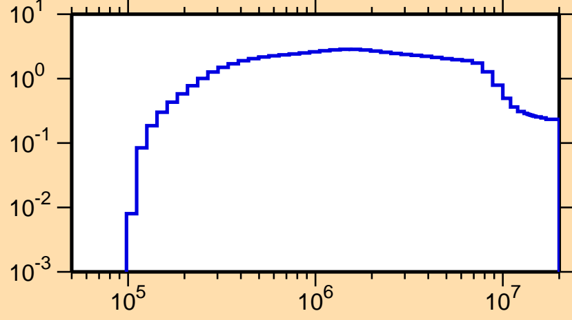
\sigma vs. E for ^{248}\text{Md}(n,\text{inel.})
