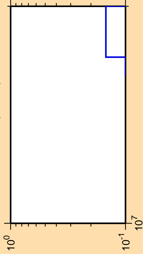
\Delta\sigma/\sigma vs. E for ^{248}\text{Md} (mt 42)
