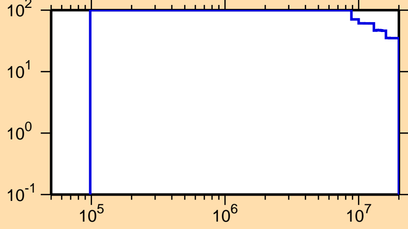
\Delta\sigma/\sigma vs. E for ^{248}\text{Md}(n,\text{f})
