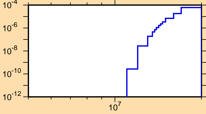
\sigma vs. E for ^{248}\text{Md}(n,2np)
