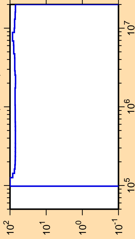
\Delta\sigma/\sigma vs. E for ^{248}\text{Md}(n,\text{inel.})
