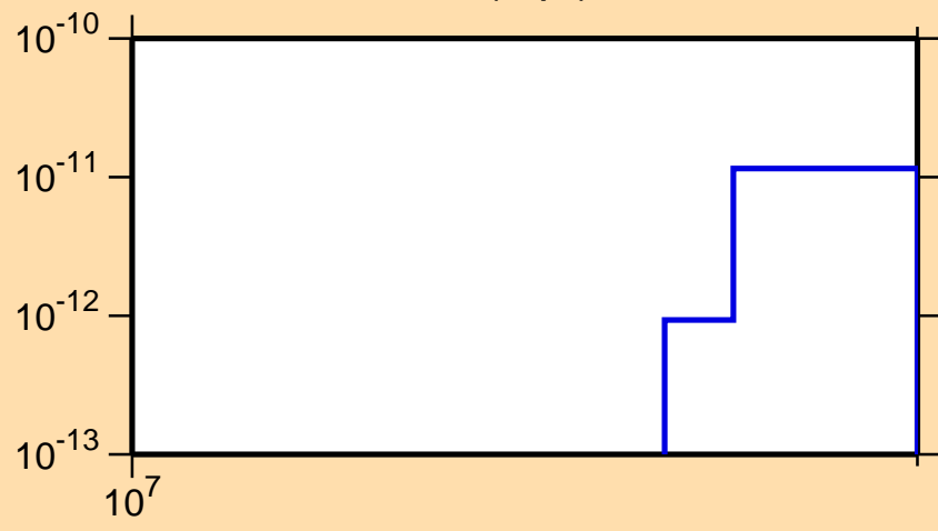
\sigma vs. E for ^{248}\text{Md}(n,\text{pt})
