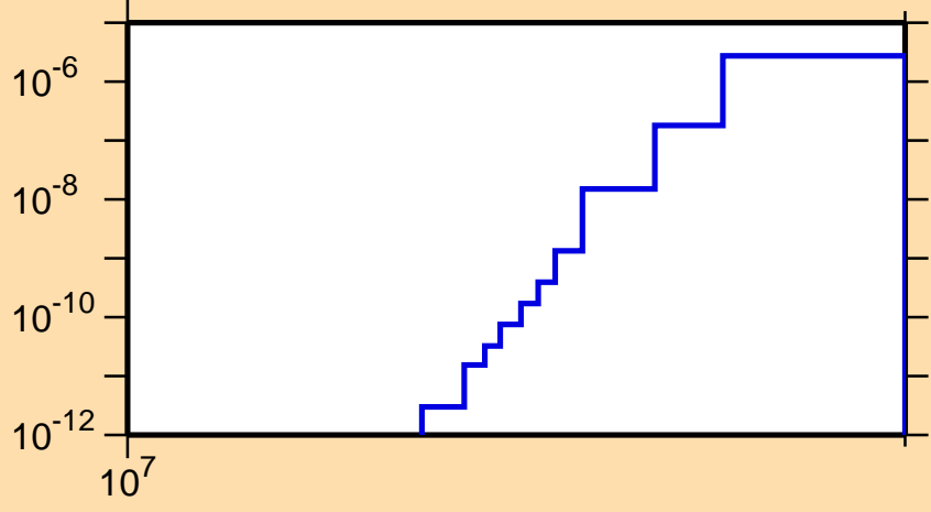
\sigma vs. E for ^{248}\text{Md}(n,nt)
