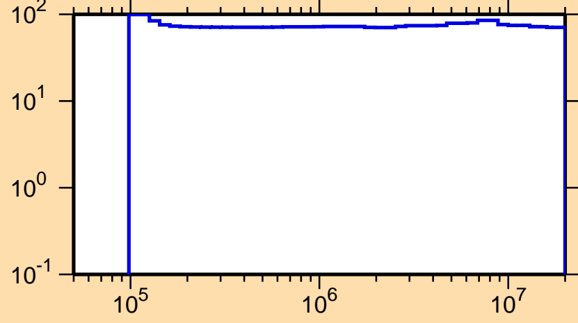
\Delta\sigma/\sigma vs. E for ^{248}\text{Md}(n,\text{inel.})
