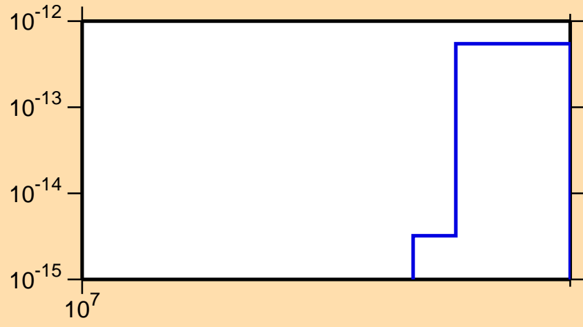
\sigma vs. E for ^{248}\text{Md}(\text{mt } 11)
