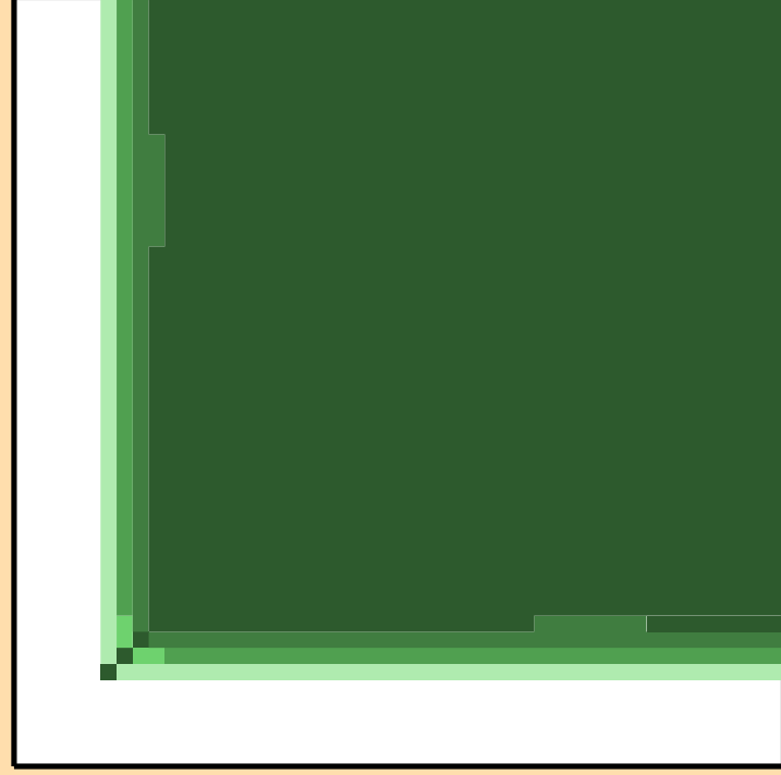
\sigma vs. E for ^{248}\text{Md}(n,n\text{cont.})
