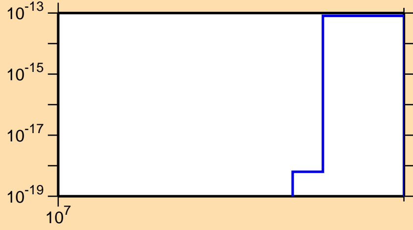
\sigma vs. E for ^{248}\text{Md} (mt 42)
