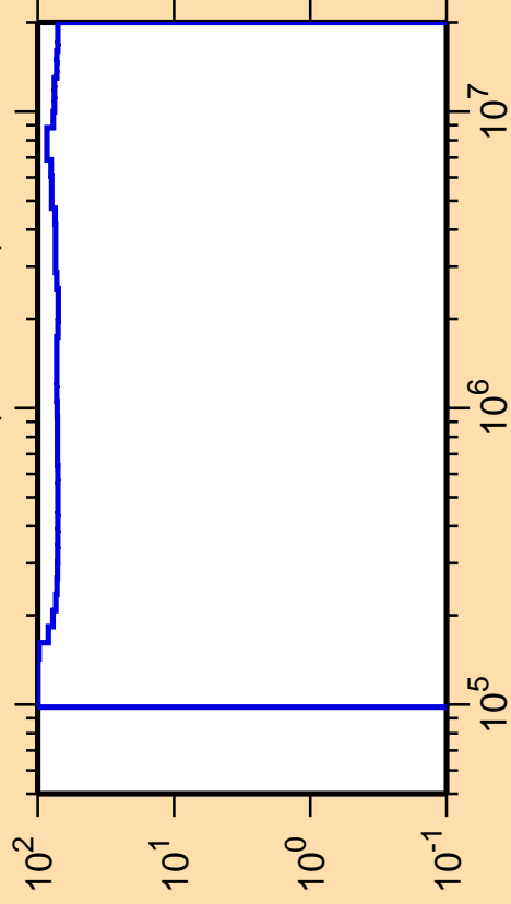
\Delta\sigma/\sigma vs. E for ^{248}\text{Md}(n,\text{ncont.})
