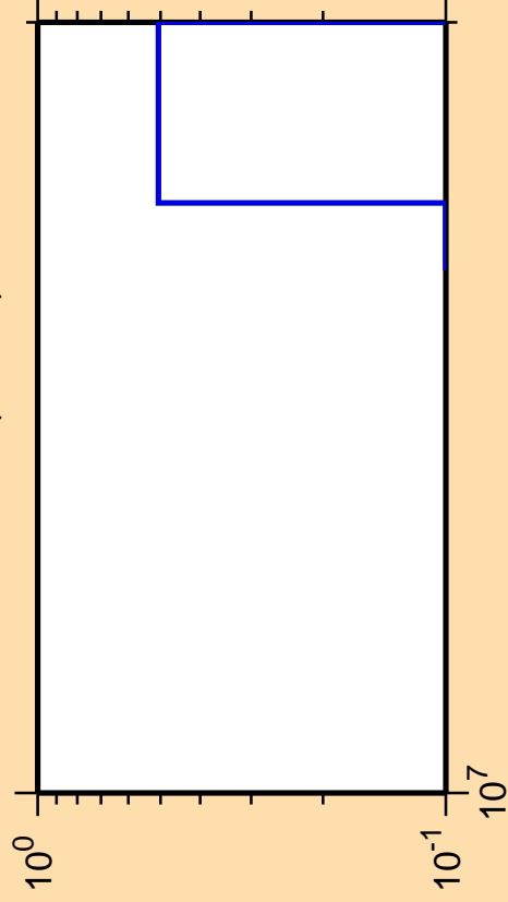
\Delta\sigma/\sigma vs. E for ^{248}\text{Md}(\text{mt } 11)
