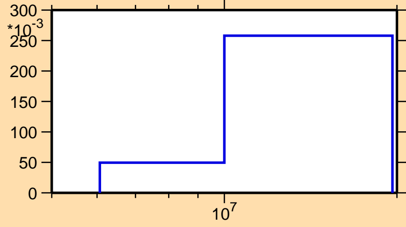
\sigma vs. E for ^{248}\text{Md}(n,2n\alpha)
