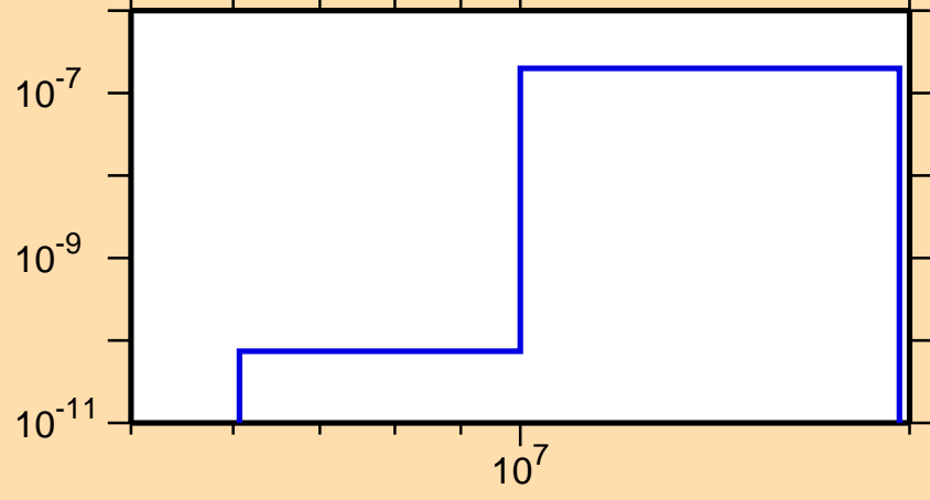
\sigma vs. E for ^{248}\text{Md}(\text{mt117})
