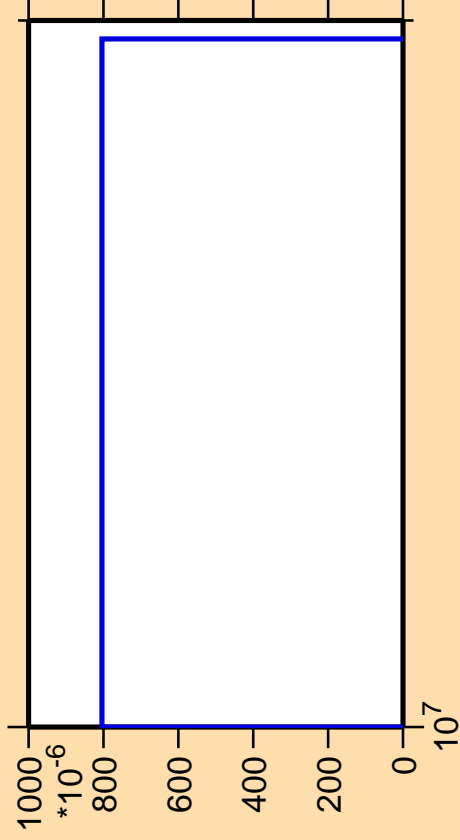
\Delta\sigma/\sigma vs. E for ^{248}\text{Md} (mt 42)
