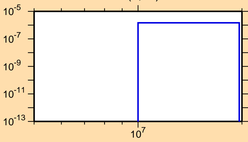
\sigma vs. E for ^{248}\text{Md}(n,\text{nd})
