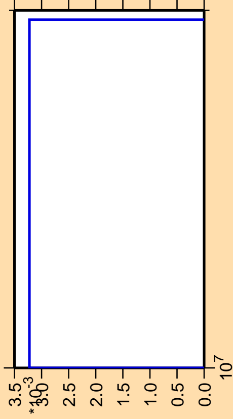
\Delta\sigma/\sigma vs. E for ^{248}\text{Md} (mt 11)
