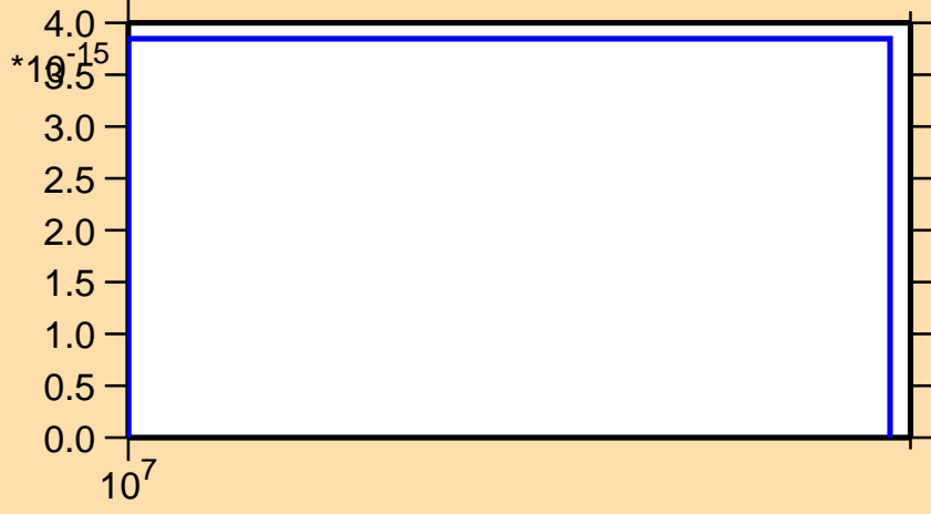
\sigma vs. E for ^{248}\text{Md} (mt 11)
