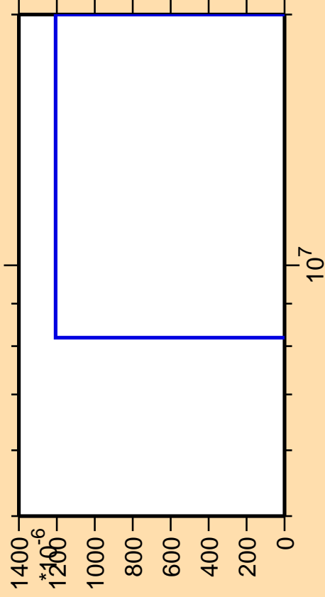
\Delta\sigma/\sigma vs. E for ^{248}\text{Md}(\text{mt } 42)
