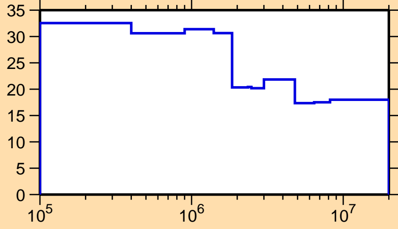
\Delta\sigma/\sigma vs. E for ^{248}\text{Md}(n,n\text{onel.})
