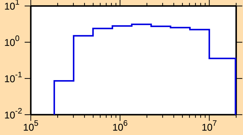
\sigma vs. E for ^{249}\text{Md}(n,\text{inel.})
