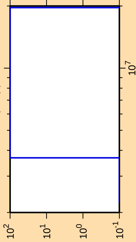
\Delta\sigma/\sigma vs. E for ^{249}\text{Md}(n,np)
