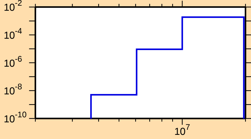
\sigma vs. E for ^{249}\text{Md}(n,np)
