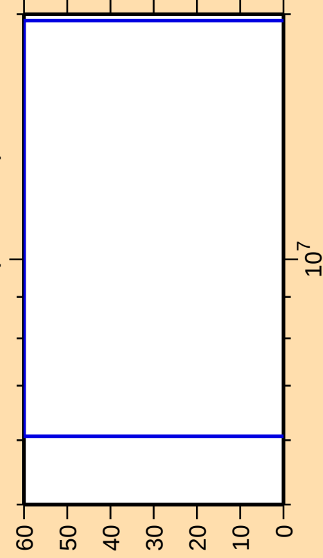
\Delta\sigma/\sigma vs. E for ^{249}\text{Md}(n,\text{ncont.})
