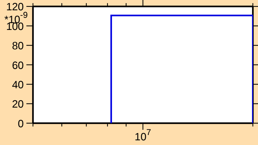
\sigma vs. E for ^{249}\text{Md}(n,\text{nd})
