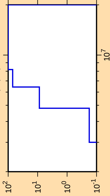
\Delta\sigma/\sigma vs. E for ^{249}\text{Md}(n,p\alpha)
