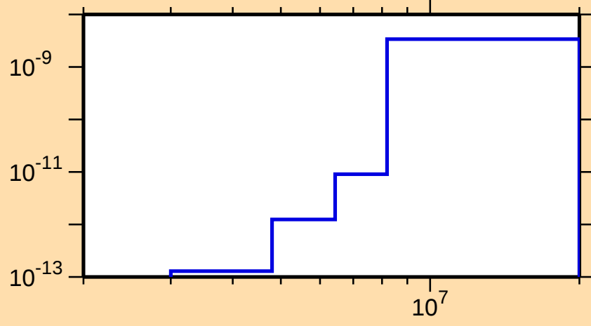
\sigma vs. E for ^{249}\text{Md}(n,p\alpha)
