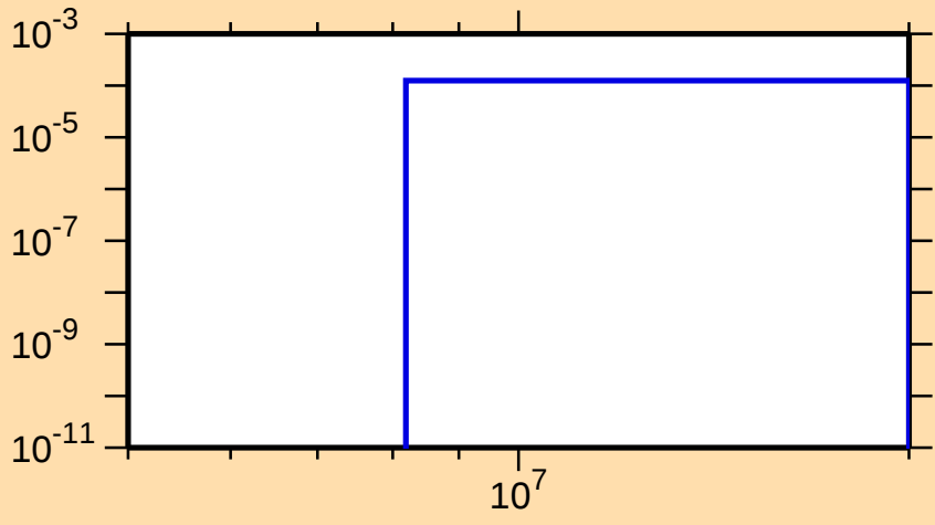
\sigma vs. E for ^{249}\text{Md}(n,t)
