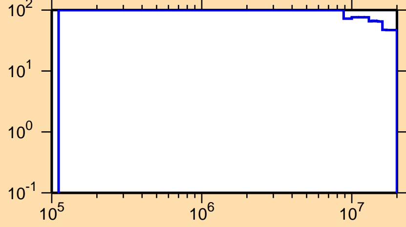
\Delta\sigma/\sigma vs. E for ^{249}\text{Md}(n,\text{f})
