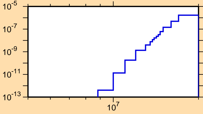
\sigma vs. E for ^{249}\text{Md} (mt 45)
