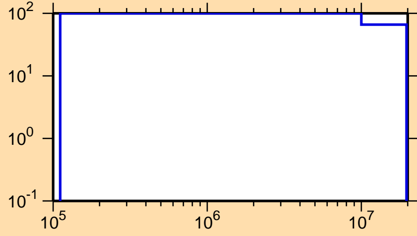
\Delta\sigma/\sigma vs. E for ^{249}\text{Md}(n,\text{f})
