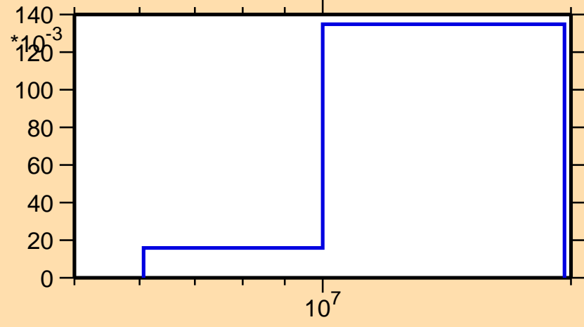
\sigma vs. E for ^{249}\text{Md}(n,2n\alpha)
