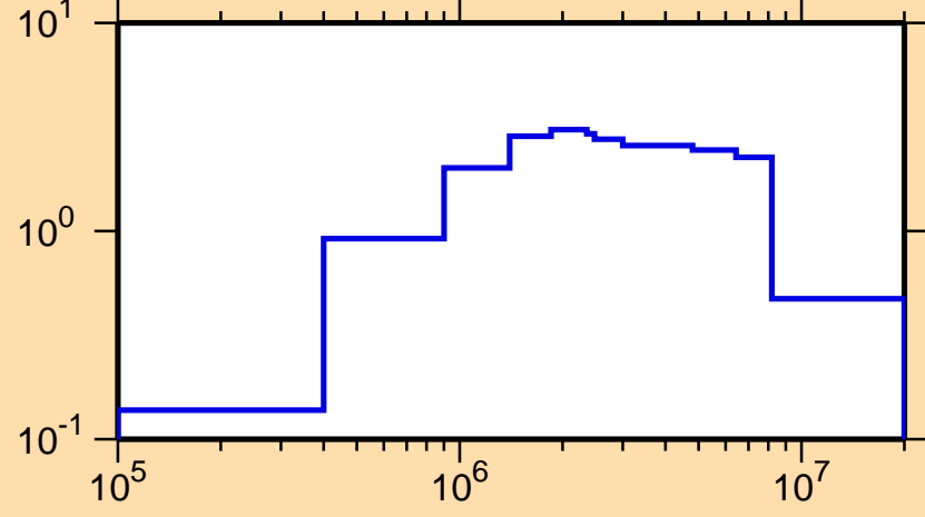
\sigma vs. E for ^{249}\text{Md}(n,n\text{cont.})
