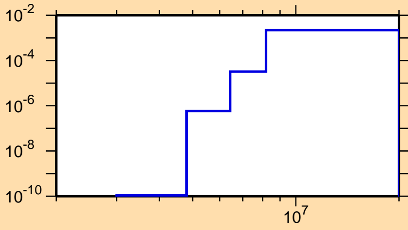
\sigma vs. E for ^{249}\text{Md}(n,np)
