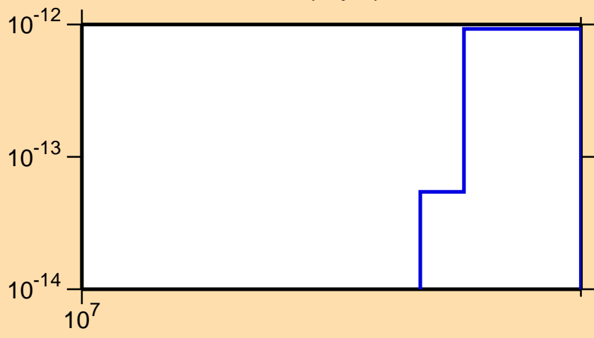
\sigma vs. E for ^{250}\text{Md}(n,\text{pd})
