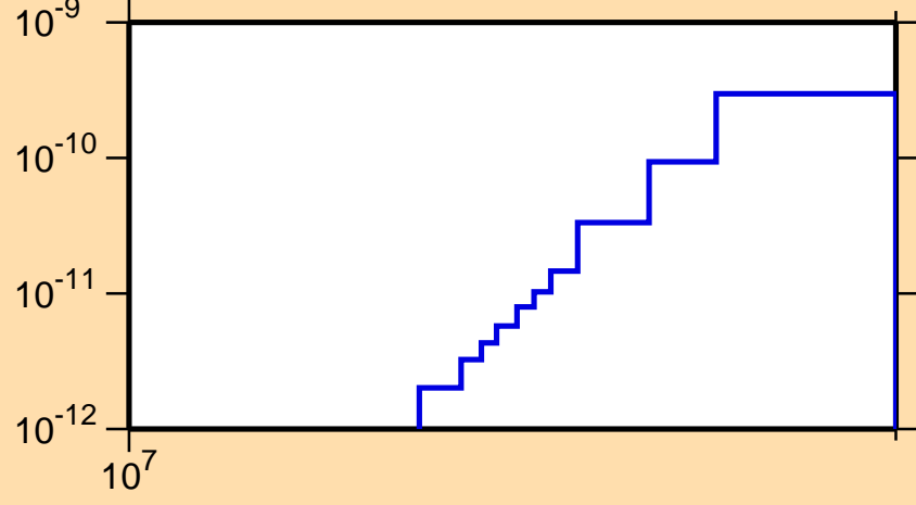
\sigma vs. E for ^{250}\text{Md} (mt 45)
