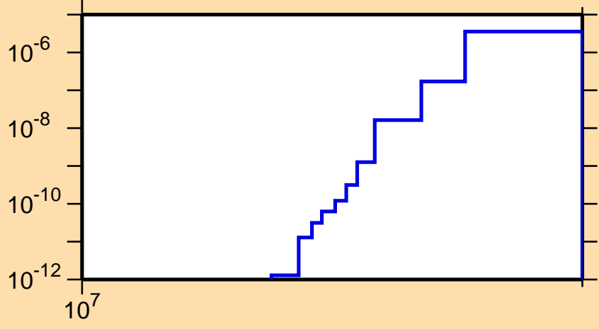
\sigma vs. E for ^{250}\text{Md}(n,nt)
