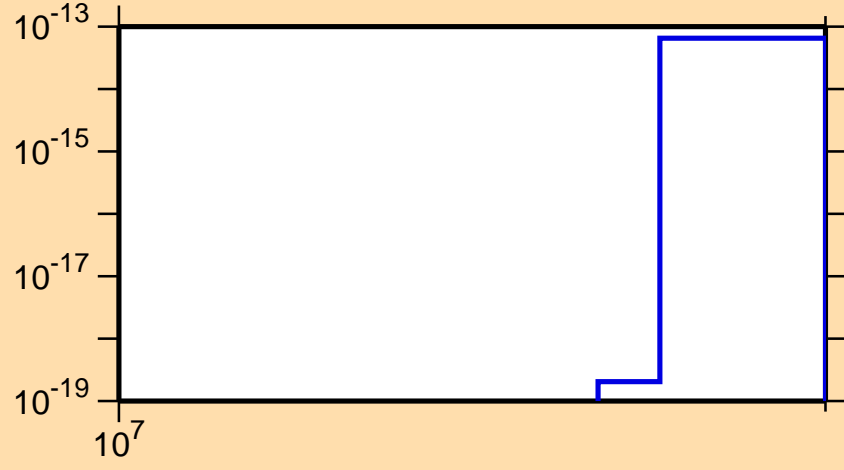
\sigma vs. E for ^{250}\text{Md} (mt 42)
