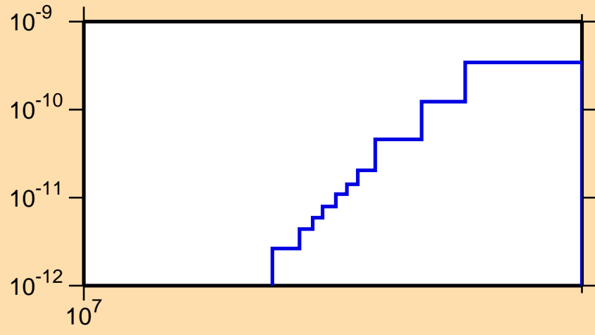
\sigma vs. E for ^{250}\text{Md}(\text{mt117})
