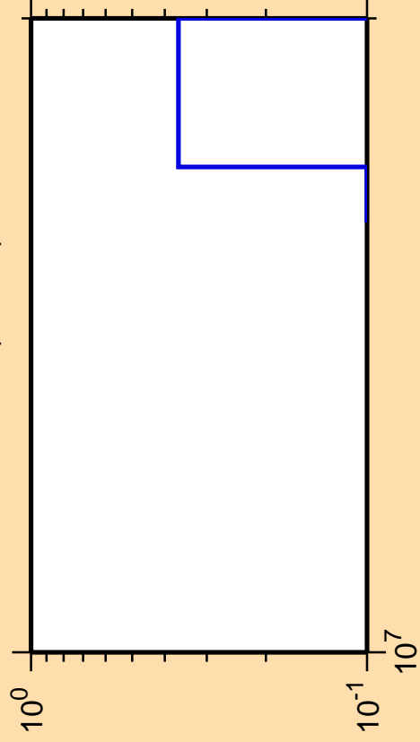
\Delta\sigma/\sigma vs. E for ^{250}\text{Md} (mt 42)
