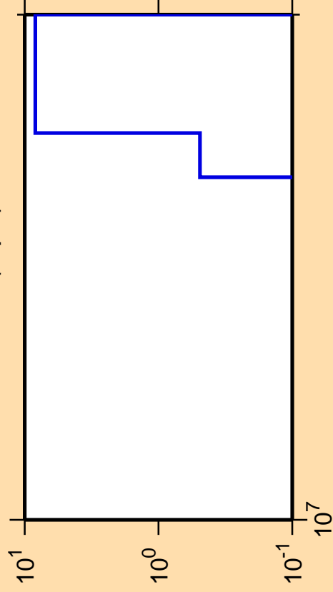
\Delta\sigma/\sigma vs. E for ^{250}\text{Md}(n,\text{pd})
