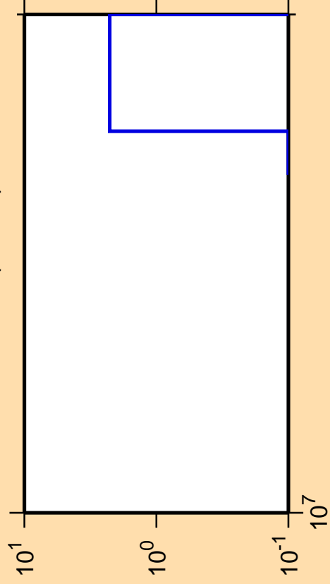
\Delta\sigma/\sigma vs. E for ^{250}\text{Md} (mt 11)
