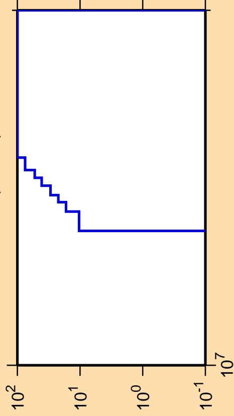
\Delta\sigma/\sigma vs. E for ^{250}\text{Md} (mt 45)
