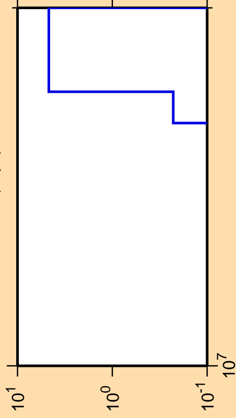
\Delta\sigma/\sigma vs. E for ^{250}\text{Md}(n,\text{pt})
