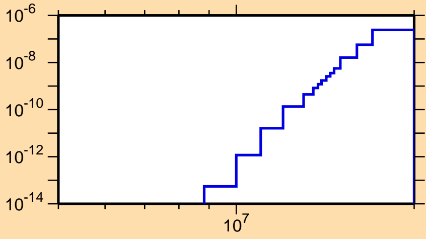
\sigma vs. E for ^{250}\text{Md}(n,\text{He}3)
