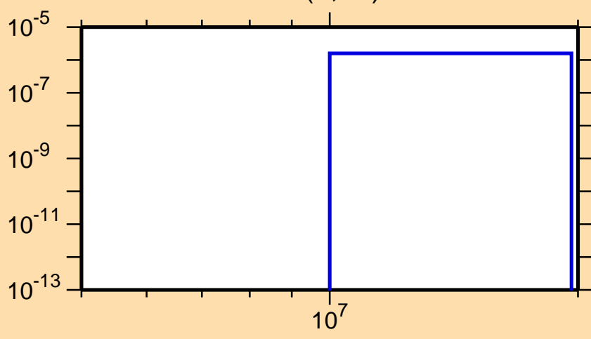
\sigma vs. E for ^{250}\text{Md}(n,\text{nd})
