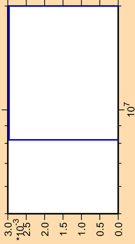
\Delta\sigma/\sigma vs. E for ^{250}\text{Md} (mt 42)
