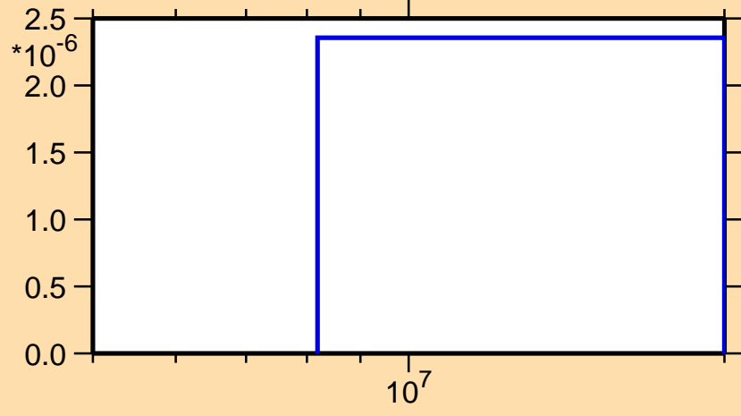
\sigma vs. E for ^{250}\text{Md}(n,2np)
