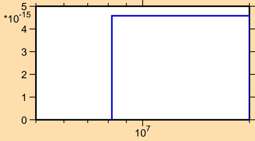
\sigma vs. E for ^{250}\text{Md}(\text{mt } 11)
