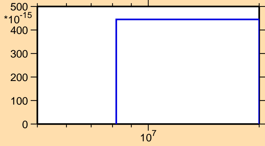
\sigma vs. E for ^{250}\text{Md}(\text{mt } 34)
