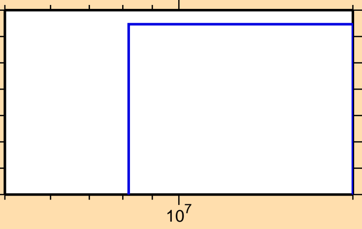
\sigma vs. E for ^{250}\text{Md}(n,\text{nd})
