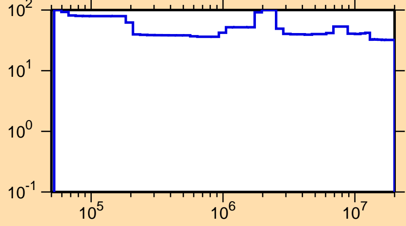
\Delta\sigma/\sigma vs. E for ^{251}\text{Md}(n,\text{inel.})
