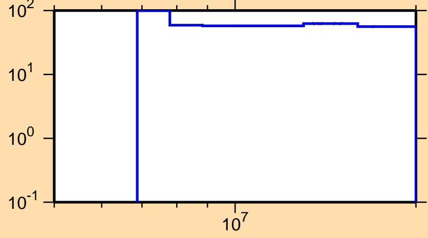
\Delta\sigma/\sigma vs. E for ^{251}\text{Md}(n,2n)
