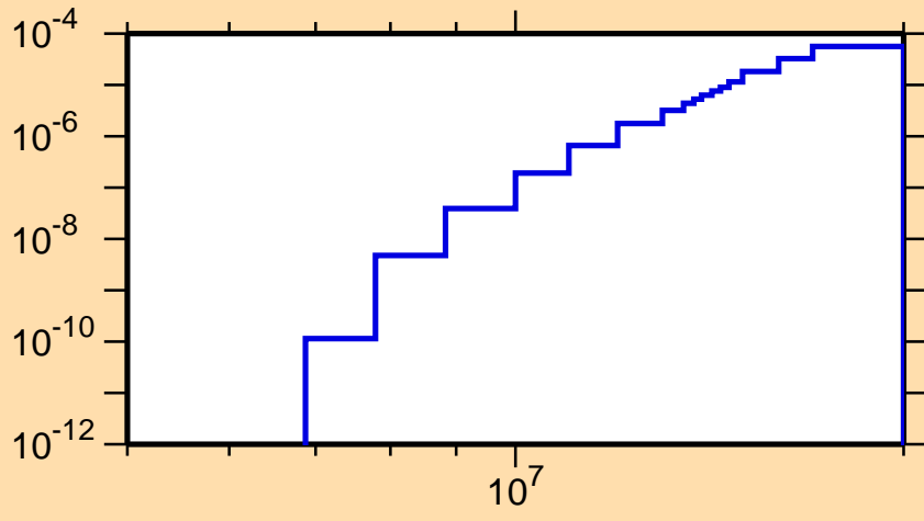
\sigma vs. E for ^{251}\text{Md}(\text{mt } 45)
