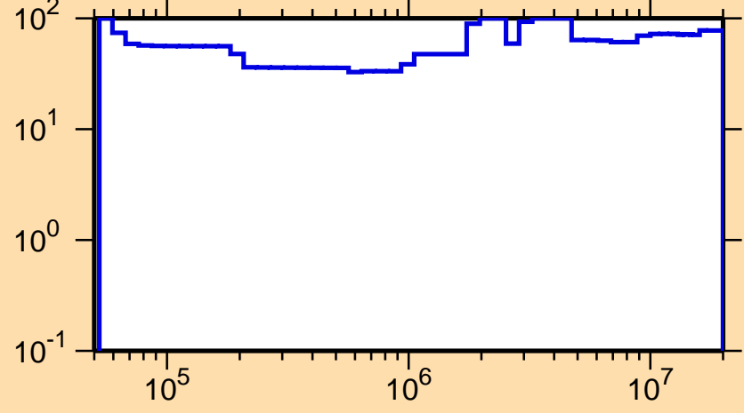
\Delta\sigma/\sigma vs. E for ^{251}\text{Md}(n,n_1)
