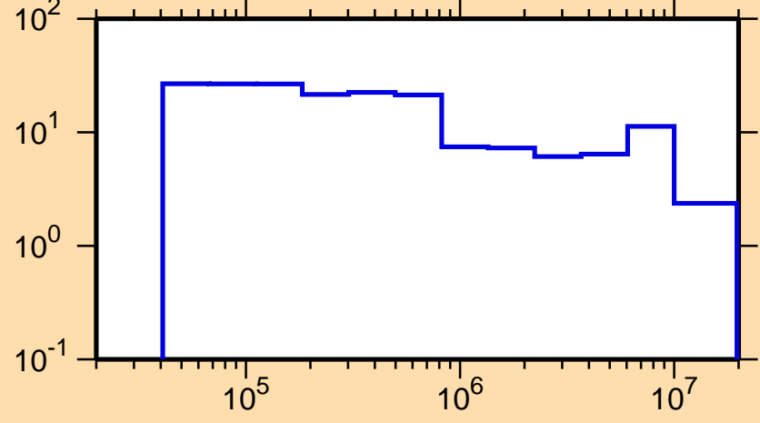
\Delta\sigma/\sigma vs. E for ^{251}\text{Md}(n,\text{tot.})
