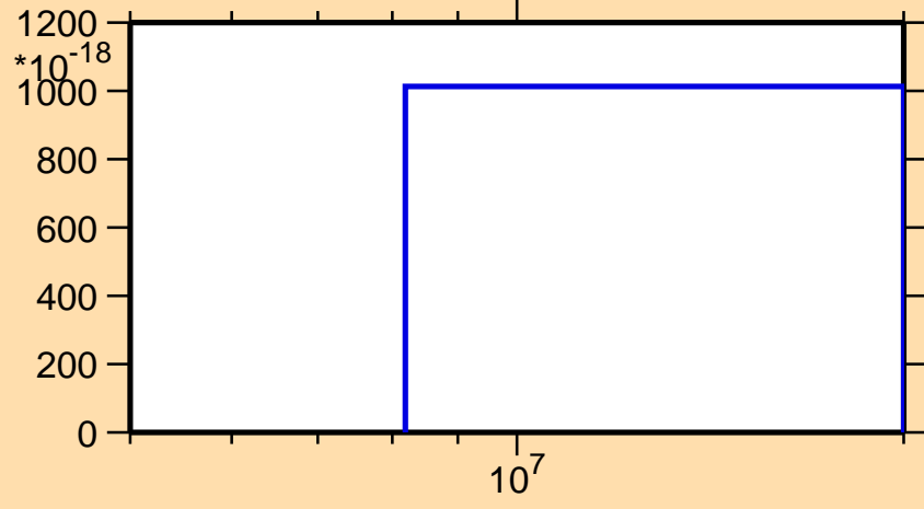
\sigma vs. E for ^{251}\text{Md} (mt 42)
