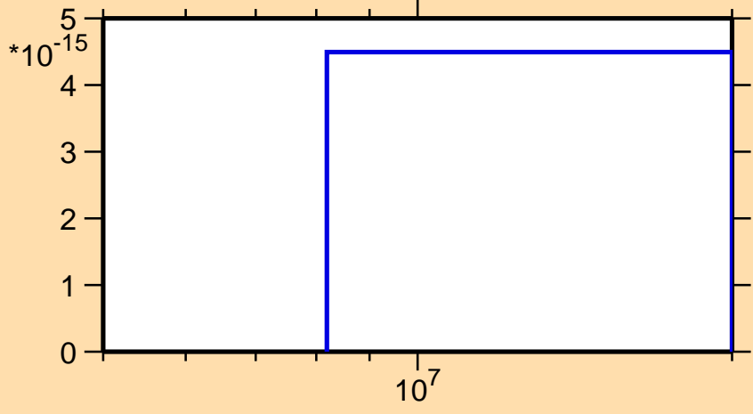
\sigma vs. E for ^{251}\text{Md}(\text{mt } 11)
