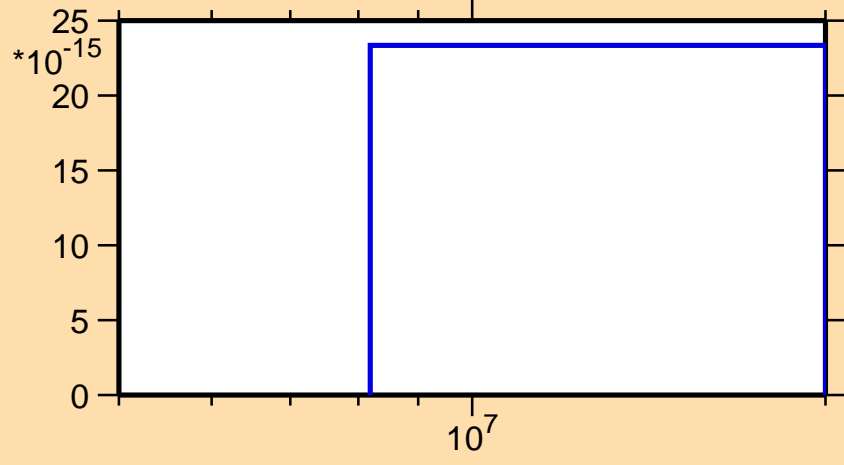
\sigma vs. E for ^{251}\text{Md}(\text{mt } 34)
