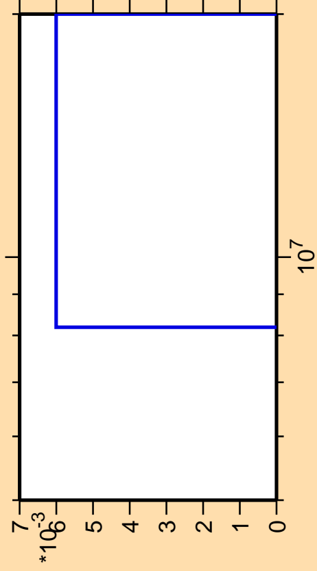
\Delta\sigma/\sigma vs. E for ^{251}\text{Md} (mt 42)
