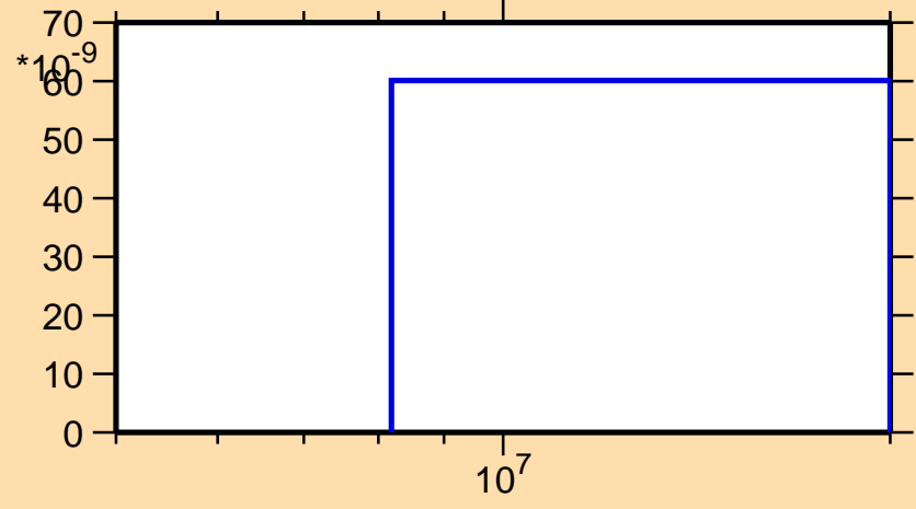
\sigma vs. E for ^{251}\text{Md}(n,nt)
