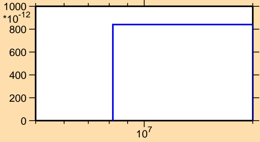
\sigma vs. E for ^{251}\text{Md}(n,\text{He3})
