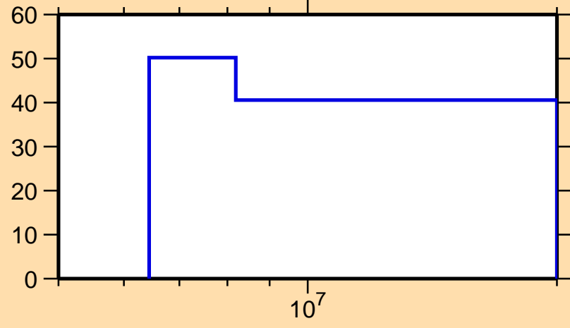
\Delta\sigma/\sigma vs. E for ^{251}\text{Md}(n,\text{inel.})
