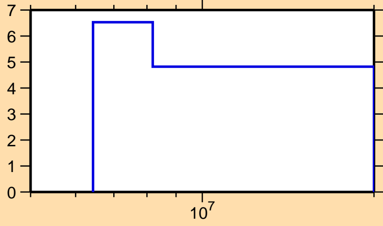
\Delta\sigma/\sigma vs. E for ^{251}\text{Md}(n,\text{nonel.})
