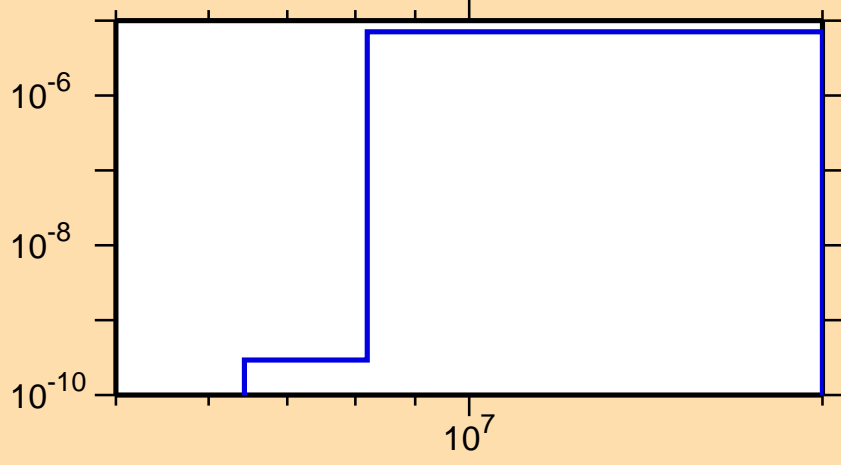
\sigma vs. E for ^{251}\text{Md}(\text{mt } 45)
