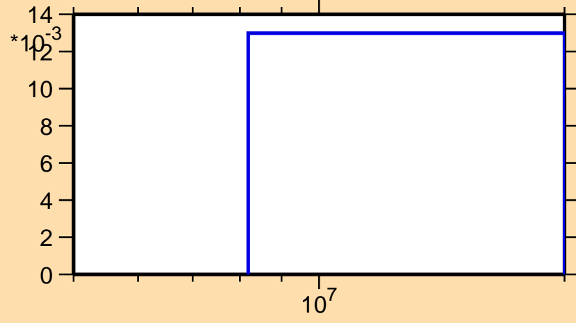
\sigma vs. E for ^{251}\text{Md}(n,3n)
