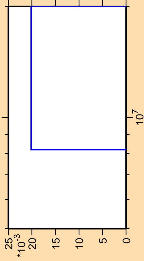
\Delta\sigma/\sigma vs. E for ^{251}\text{Md}(\text{mt } 34)
