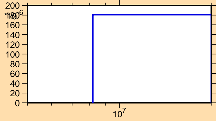
\sigma vs. E for ^{251}\text{Md}(n,3n\alpha)
