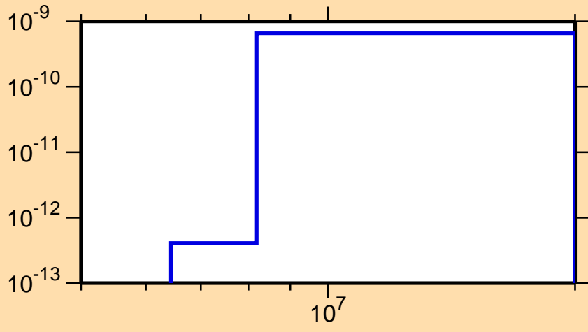
\sigma vs. E for ^{251}\text{Md}(n,p\alpha)
