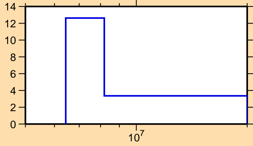
\Delta\sigma/\sigma vs. E for ^{251}\text{Md}(n,\text{tot.})
