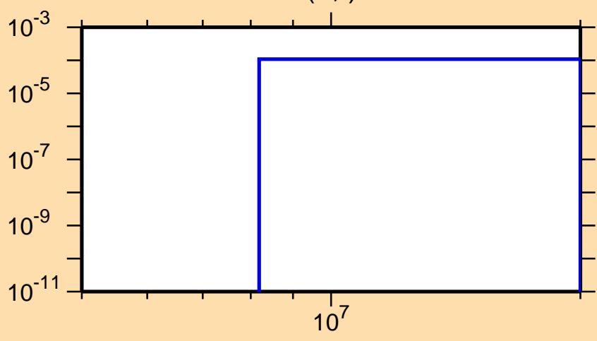
\sigma vs. E for ^{251}\text{Md}(n,t)
