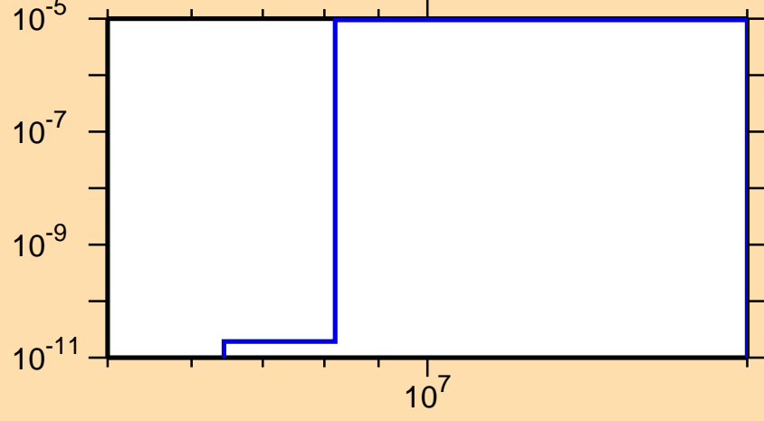
\sigma vs. E for ^{251}\text{Md}(\text{mt117})
