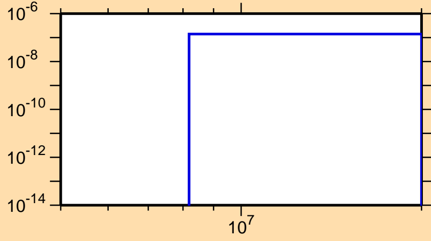
\sigma vs. E for ^{251}\text{Md}(n,\text{nd})
