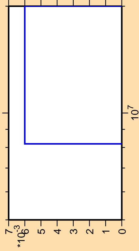
\Delta\sigma/\sigma vs. E for ^{251}\text{Md}(\text{mt } 11)
