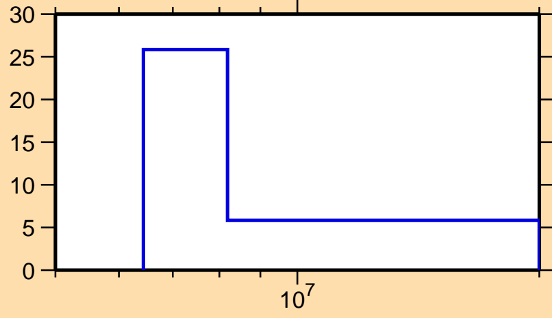
\Delta\sigma/\sigma vs. E for ^{251}\text{Md}(n,\text{el.})
