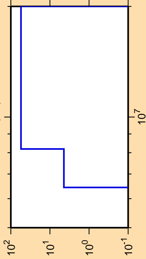
\Delta\sigma/\sigma vs. E for ^{251}\text{Md}(n,t)
