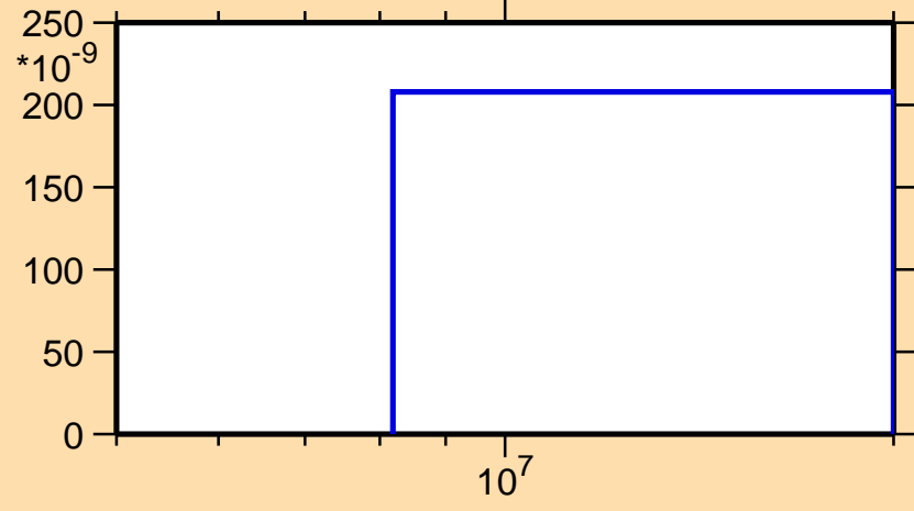
\sigma vs. E for ^{251}\text{Md}(n,2np)
