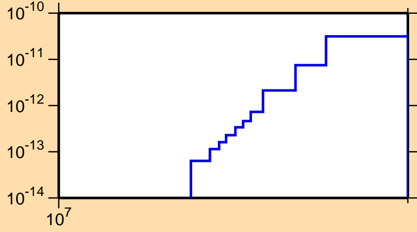
\sigma vs. E for ^{252}\text{Md}(\text{mt } 45)
