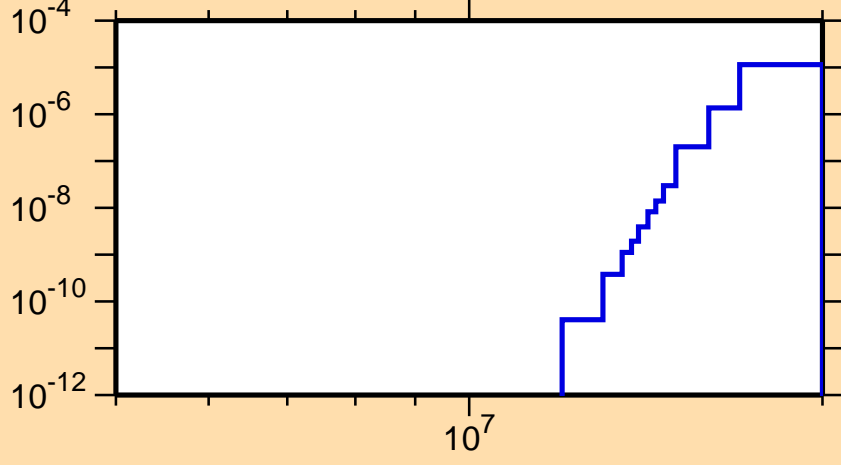
\sigma vs. E for ^{252}\text{Md}(n,\text{nd})
