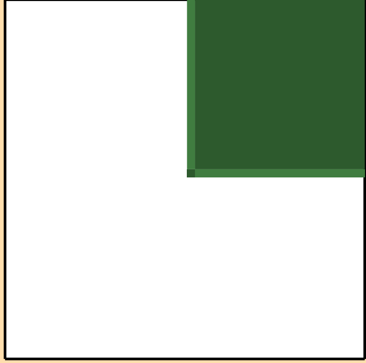
\sigma vs. E for ^{252}\text{Md}(n,3n)
