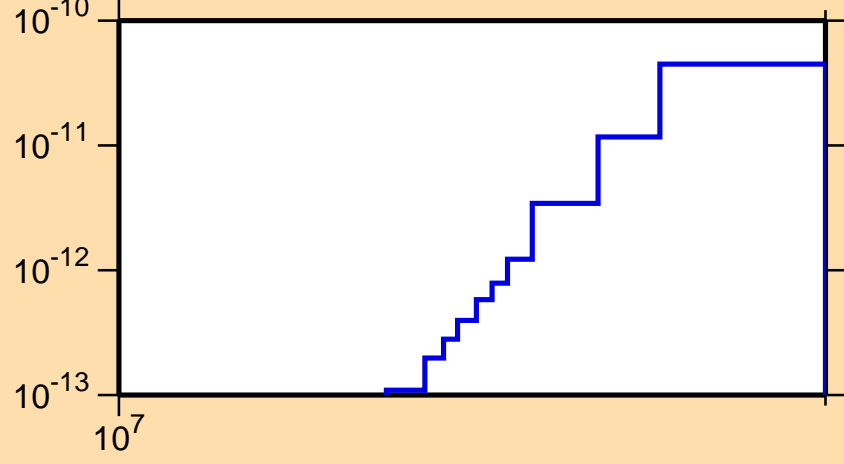
\sigma vs. E for ^{252}\text{Md}(\text{mt117})
