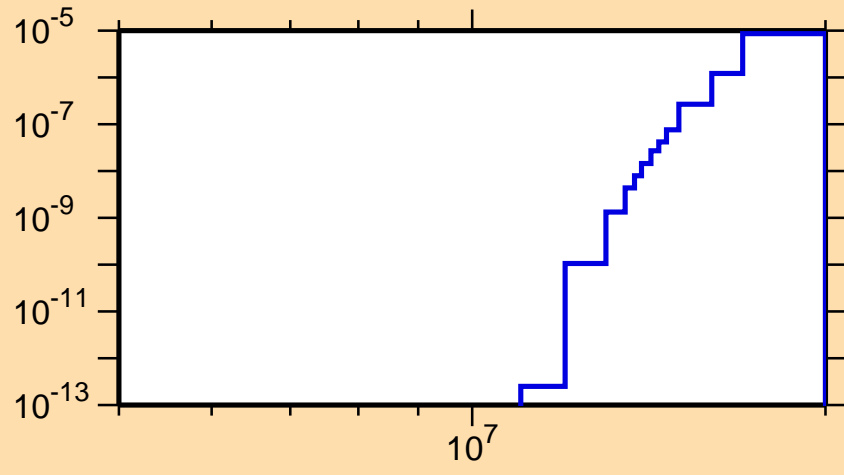
\sigma vs. E for ^{252}\text{Md}(n,2np)
