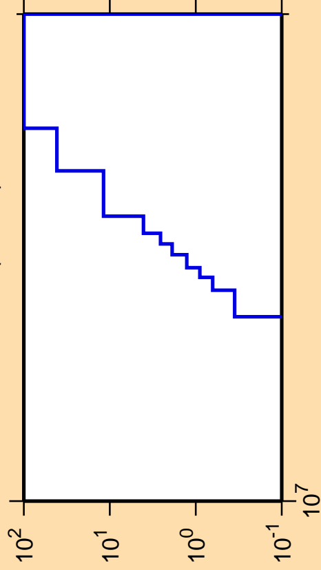
\Delta\sigma/\sigma vs. E for ^{252}\text{Md}(\text{mt } 45)
