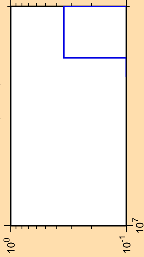
\Delta\sigma/\sigma vs. E for ^{252}\text{Md} (mt 42)
