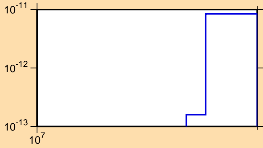
\sigma vs. E for ^{252}\text{Md} (mt 34)
