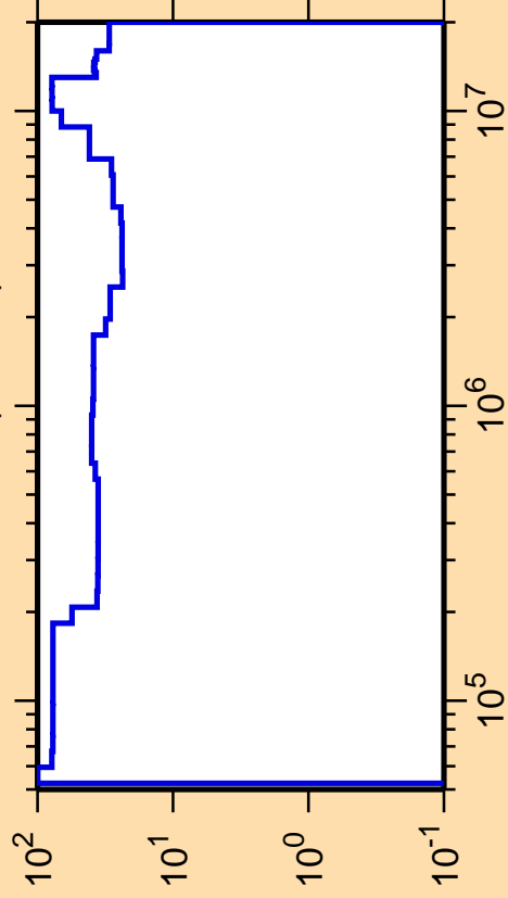
\Delta\sigma/\sigma vs. E for ^{252}\text{Md}(n,\text{inel.})
