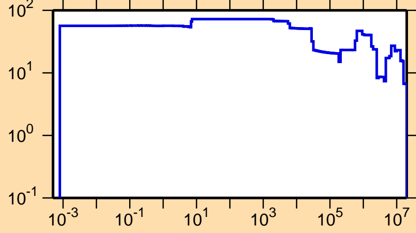
\Delta\sigma/\sigma vs. E for ^{252}\text{Md}(n,\text{el.})
