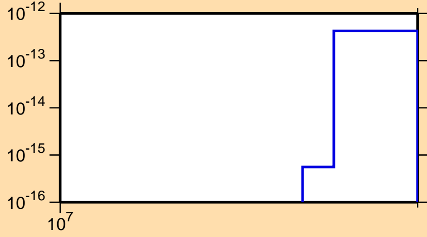
\sigma vs. E for ^{252}\text{Md} (mt 11)
