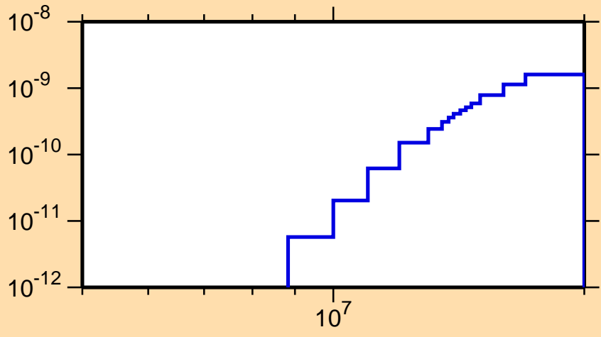
\sigma vs. E for ^{252}\text{Md}(n,p\alpha)
