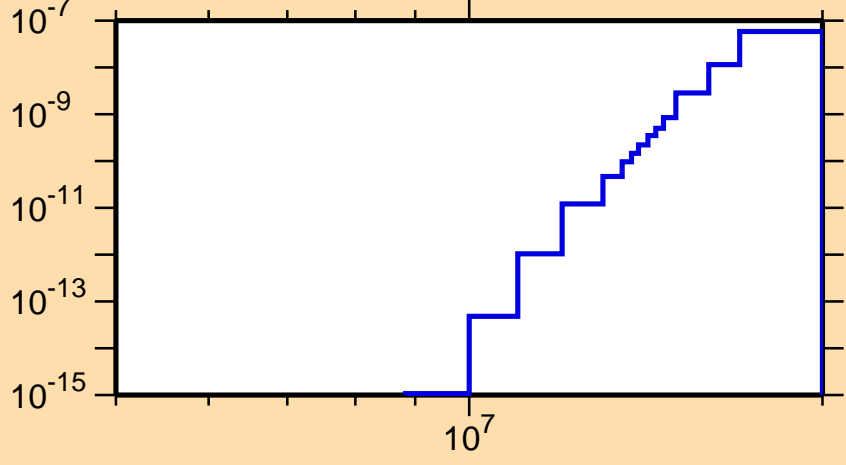
\sigma vs. E for ^{252}\text{Md}(n,\text{He3})
