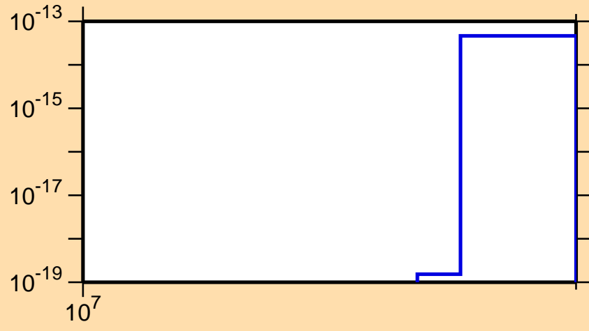
\sigma vs. E for ^{252}\text{Md} (mt 42)
