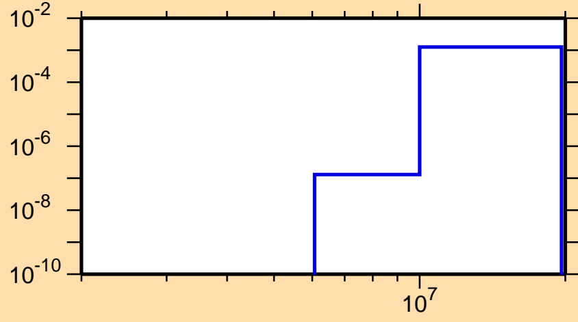
\sigma vs. E for ^{252}\text{Md}(n,d)
