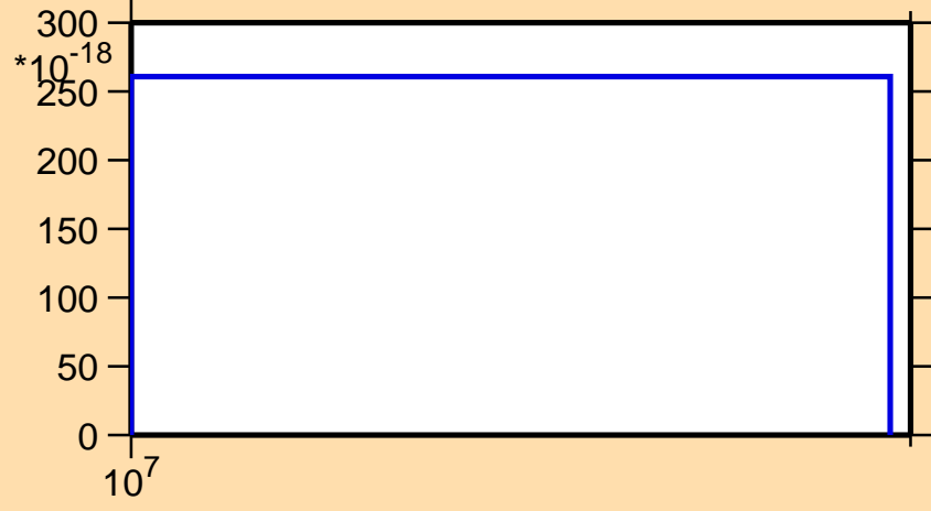
\sigma vs. E for ^{252}\text{Md} (mt 42)
