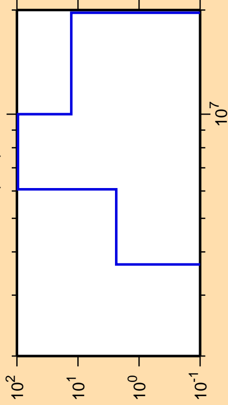
\Delta\sigma/\sigma vs. E for ^{252}\text{Md}(n,d)
