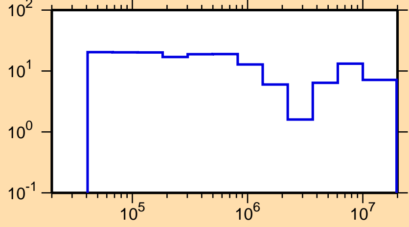
\Delta\sigma/\sigma vs. E for ^{252}\text{Md}(n,\text{tot.})
