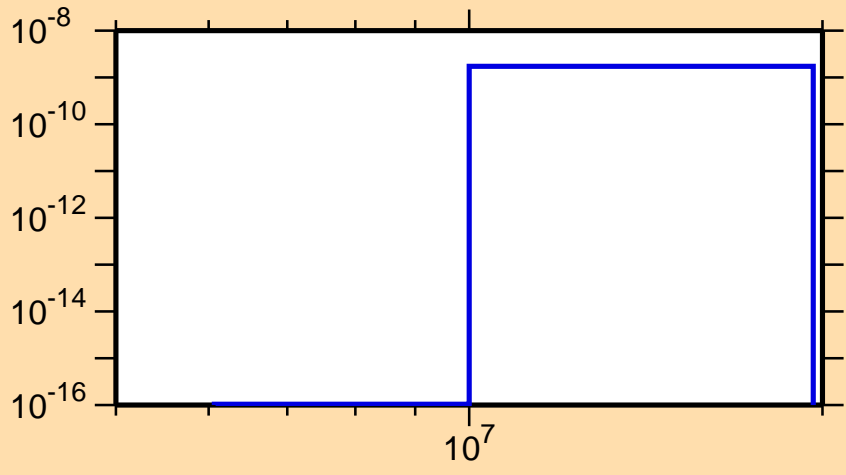
\sigma vs. E for ^{252}\text{Md}(n,\text{He3})
