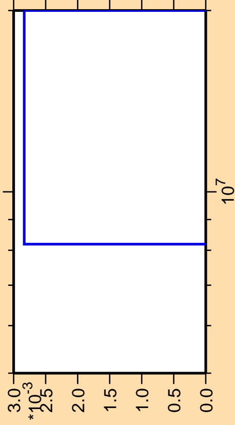
\Delta\sigma/\sigma vs. E for ^{252}\text{Md} (mt 42)
