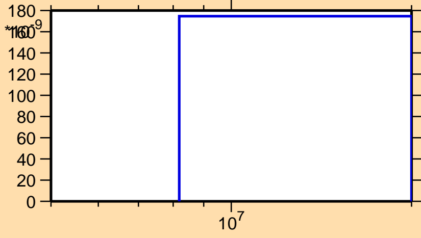
\sigma vs. E for ^{252}\text{Md}(n,\text{nd})
