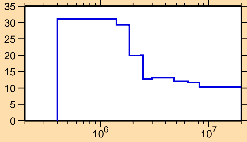
\Delta\sigma/\sigma vs. E for ^{252}\text{Md}(n,n\text{onel.})
