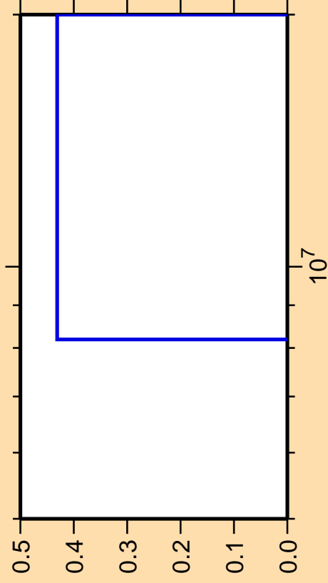
\Delta\sigma/\sigma vs. E for ^{252}\text{Md}(\text{mt } 34)
