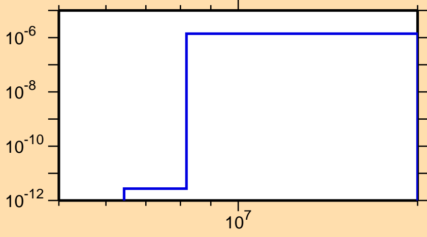
\sigma vs. E for ^{252}\text{Md}(n,2n\alpha)
