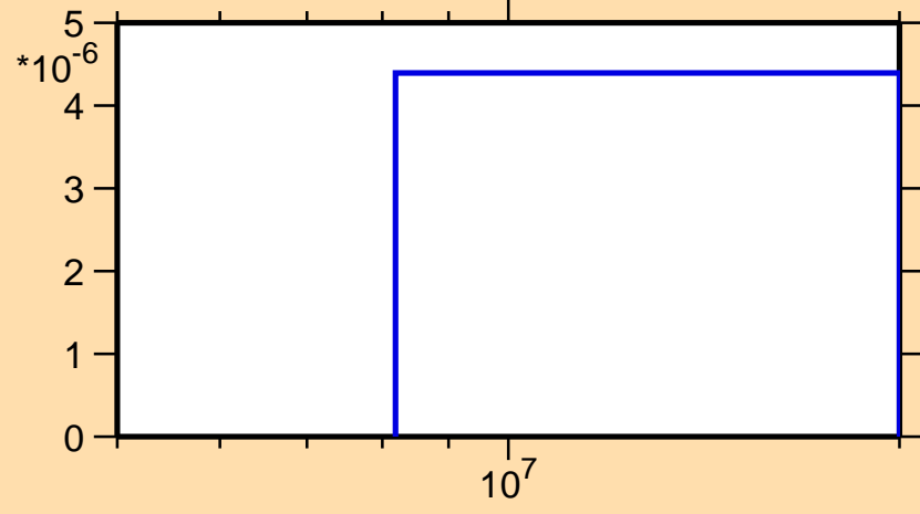
\sigma vs. E for ^{252}\text{Md}(n,3n\alpha)
