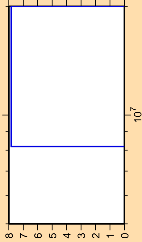
\Delta\sigma/\sigma vs. E for ^{252}\text{Md}(\text{mt117})
