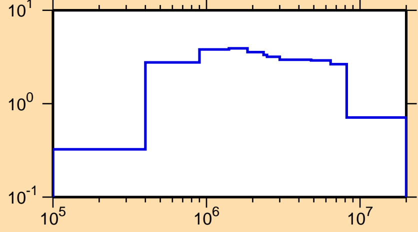
\sigma vs. E for ^{252}\text{Md}(n,\text{inel.})
