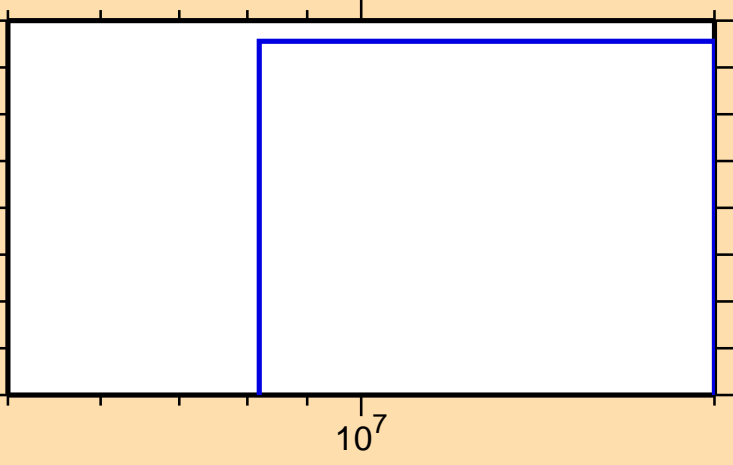
\sigma vs. E for ^{252}\text{Md} (mt 42)
