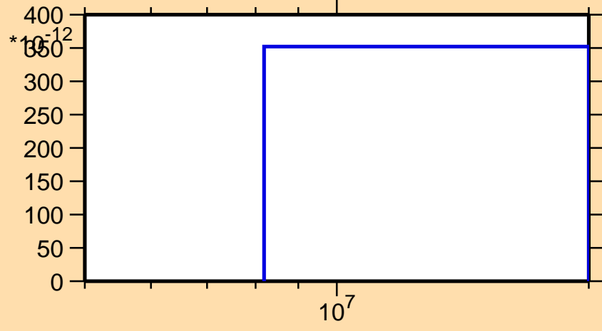
\sigma vs. E for ^{252}\text{Md}(n,p\alpha)
