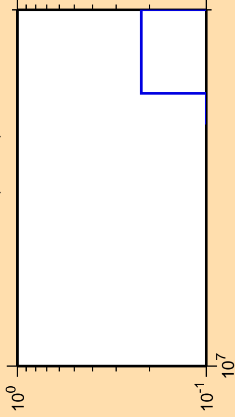
\Delta\sigma/\sigma vs. E for ^{253}\text{Md} (mt 11)
