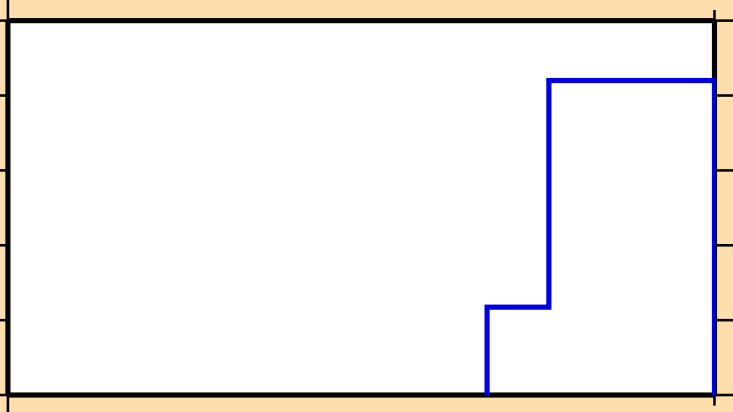
\sigma vs. E for ^{253}\text{Md} (mt 45)
