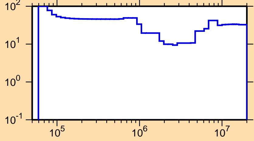
\Delta\sigma/\sigma vs. E for ^{253}\text{Md}(n,\text{inel.})
