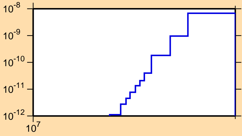
\sigma vs. E for ^{253}\text{Md}(n,\text{He}3)
