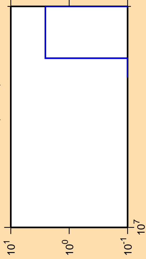
\Delta\sigma/\sigma vs. E for ^{253}\text{Md} (mt 34)
