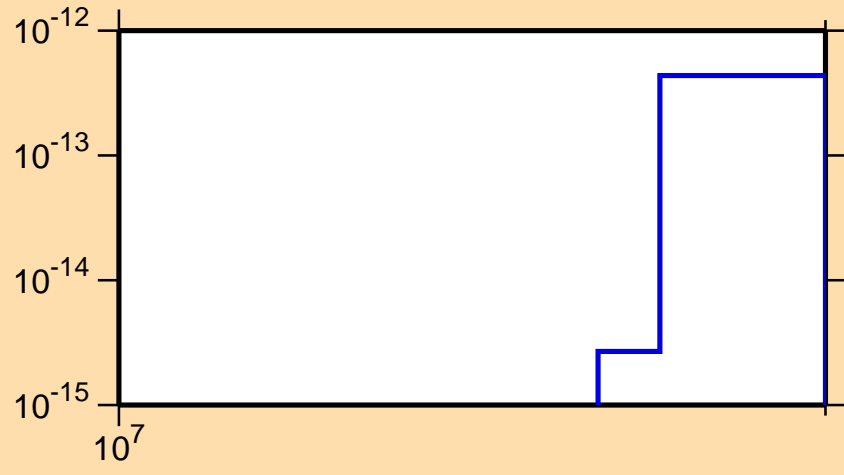
\sigma vs. E for ^{253}\text{Md} (mt 34)
