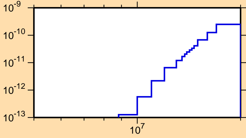
\sigma vs. E for ^{253}\text{Md}(n,p\alpha)
