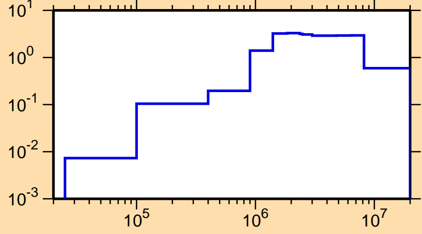
\sigma vs. E for ^{253}\text{Md}(n,\text{inel.})
