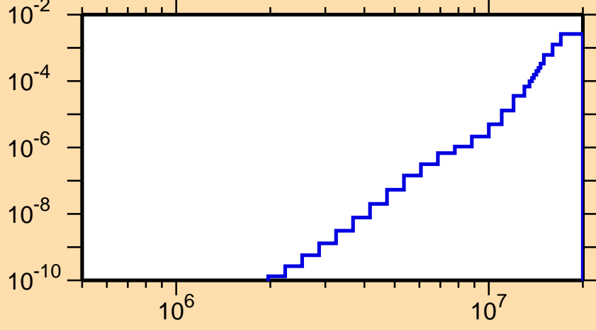
\sigma vs. E for ^{254}\text{Md}(n,\alpha)
