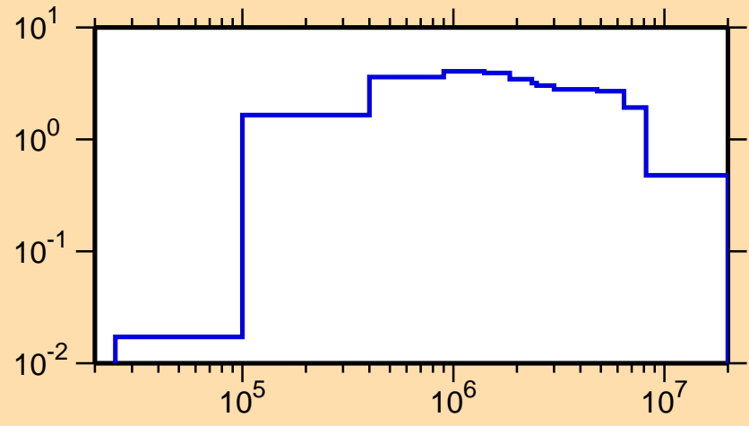
\sigma vs. E for ^{254}\text{Md}(n,\text{inel.})
