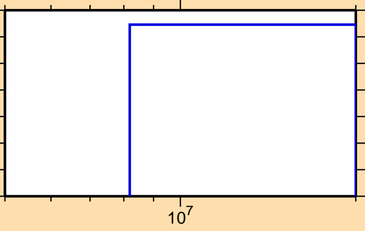
\sigma vs. E for ^{254}\text{Md}(n,\text{nd})
