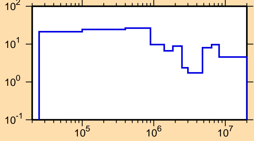
\Delta\sigma/\sigma vs. E for ^{254}\text{Md}(n,\text{tot.})
