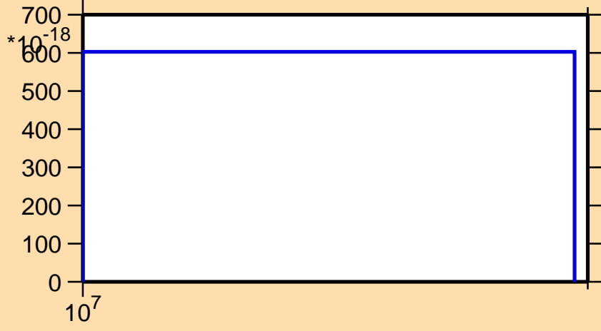
\sigma vs. E for ^{255}\text{Md} (mt 34)
