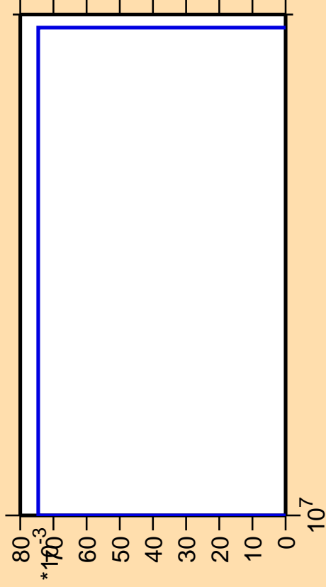
\Delta\sigma/\sigma vs. E for ^{255}\text{Md} (mt 11)
