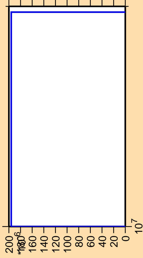
\Delta\sigma/\sigma vs. E for ^{255}\text{Md} (mt 34)
