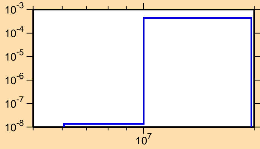
\sigma vs. E for ^{255}\text{Md}(n,d)
