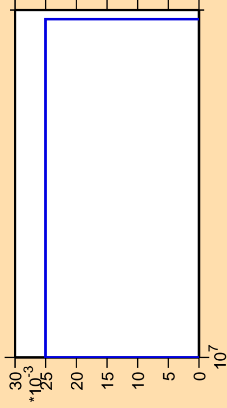
\Delta\sigma/\sigma vs. E for ^{255}\text{Md} (mt 42)
