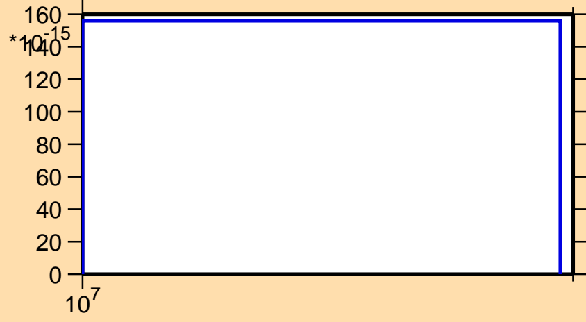
\sigma vs. E for ^{255}\text{Md} (mt 45)
