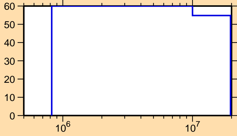
\Delta\sigma/\sigma vs. E for ^{255}\text{Md}(n,f)
