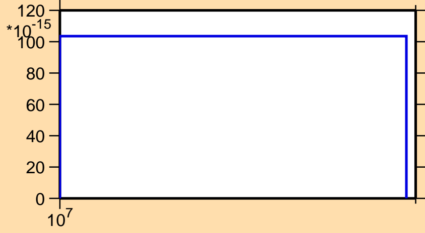
\sigma vs. E for ^{255}\text{Md} (mt 11)
