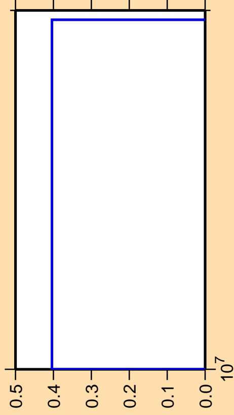
\Delta\sigma/\sigma vs. E for ^{255}\text{Md} (mt 45)
