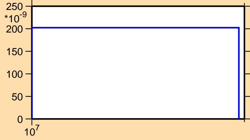
\sigma vs. E for ^{255}\text{Md}(n,\text{nd})
