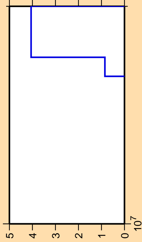
\Delta\sigma/\sigma vs. E for ^{256}\text{Md} (mt 45)
