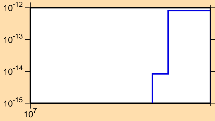
\sigma vs. E for ^{256}\text{Md}(\text{mt } 34)
