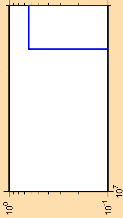
\Delta\sigma/\sigma vs. E for ^{256}\text{Md}(\text{mt } 34)
