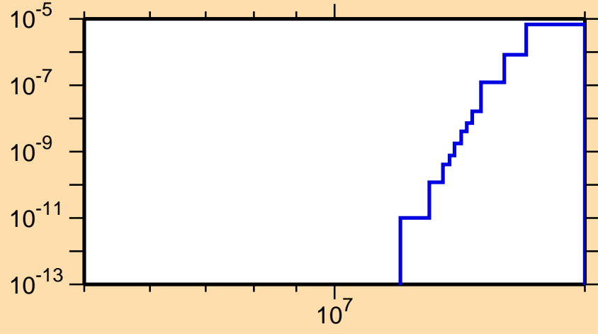
\sigma vs. E for ^{256}\text{Md}(n,2np)
