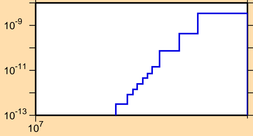
\sigma vs. E for ^{256}\text{Md}(n,\text{He3})
